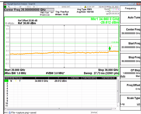
n77(3450-3550MHz) (20GHz-36GHz) 60M DFT-s-OFDM BPSK Inner 1RB Left High
