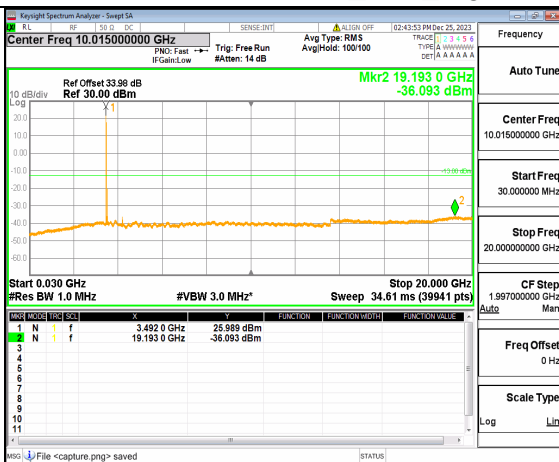
n77(3450-3550MHz) (30MHz-20GHz) 60M DFT-s-OFDM BPSK Inner 1RB Left High
