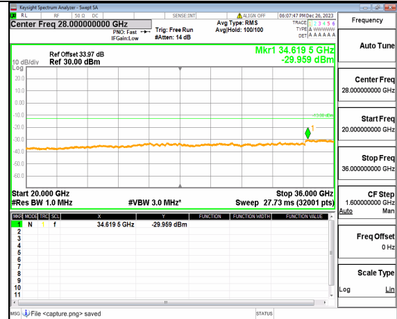
n77(3450-3550MHz) (20GHz-36GHz) 80M DFT-s-OFDM BPSK Inner_1RB_Right Low
