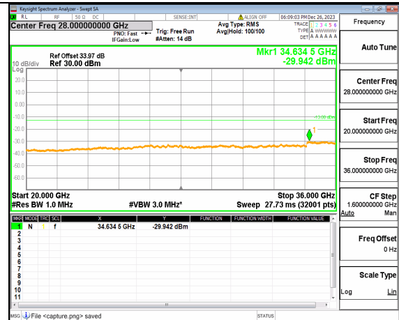
n77(3450-3550MHz) (20GHz-36GHz) 80M DFT-s-OFDM QPSK Inner_1RB_Left Low
