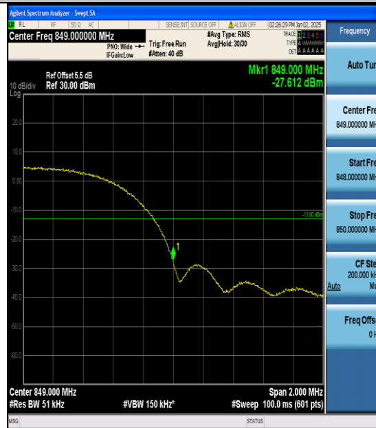
Band5-4233-1-PASS
