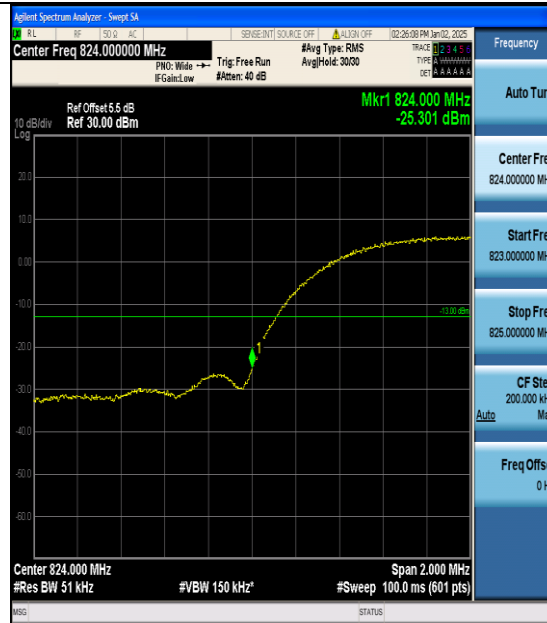
Band5-4132-1-PASS
