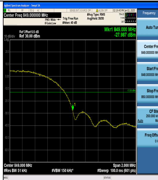
Band5-4233-1-PASS
