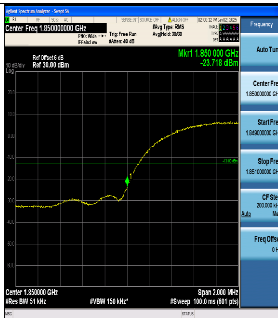
Band2-9262-1-PASS
