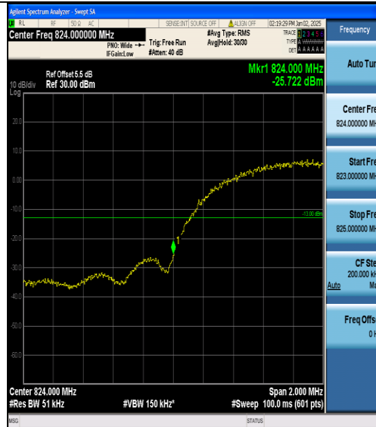
Band5-4132-1-PASS
