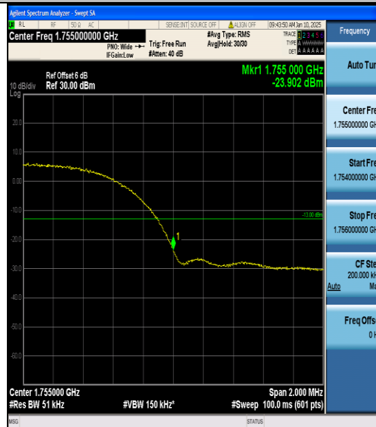
Band4-1513-1-PASS
