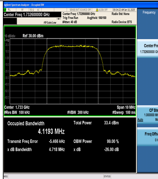
Band4-1413-1-PASS
