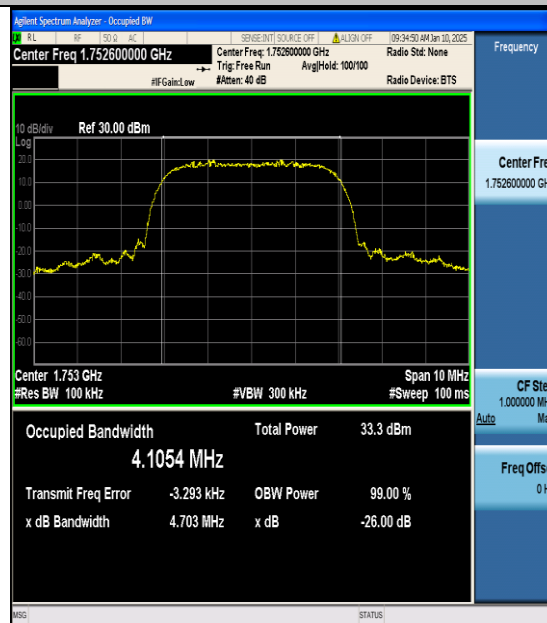
Band4-1513-1-PASS
