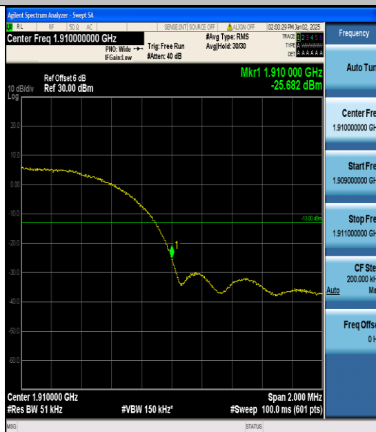
Band2-9538-1-PASS
