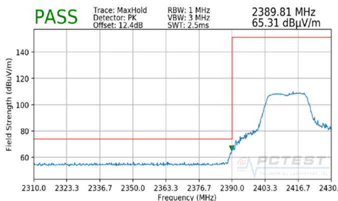
Plot 7-42. Radiated Restricted Lower Band Edge Measurement (Peak)
