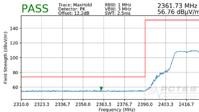
Plot 7-44. Radiated Restricted Lower Band Edge Measurement (Peak)
