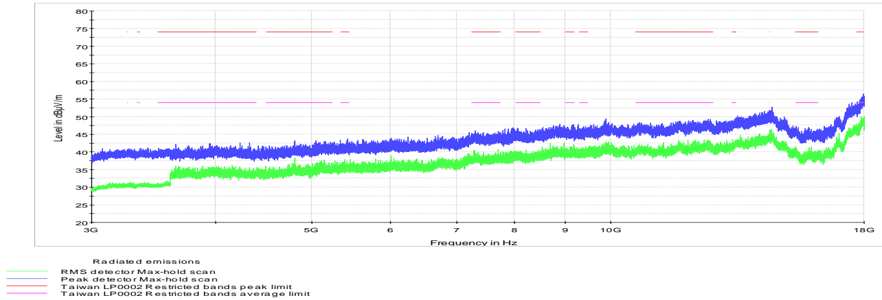
Figure 8.6-12: Radiated spurious emissions within restricted bands on low channel between 3 and 18 GHz
