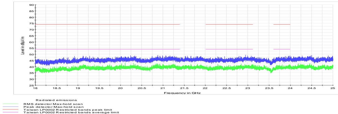
Figure 8.6-15: Radiated spurious emissions within restricted bands on low channel between 18 and 25 GHz
