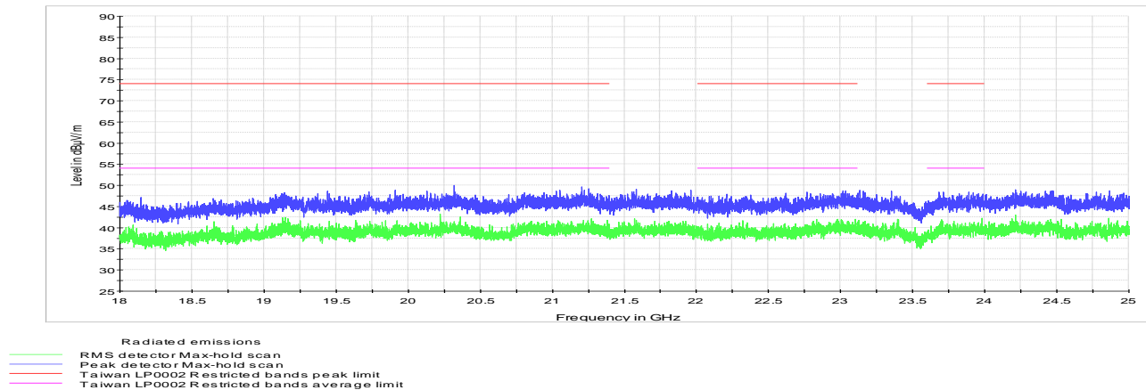
Figure 8.6-16: Radiated spurious emissions within restricted bands on mid channel between 18 and 25 GHz
