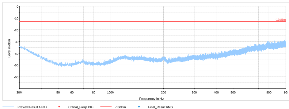
Plot #19 Radiated Emissions: 30 MHz – 1GHz
