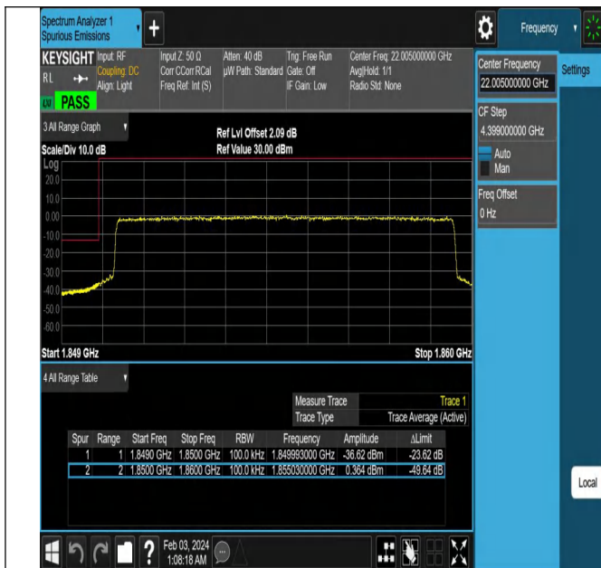
Band2_10MHz_QPSK_18650_50RB#0
