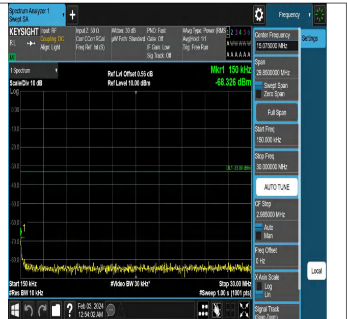
Band2_1.4MHz_QPSK_18607_1RB#0_0.15~30_0.15~30
