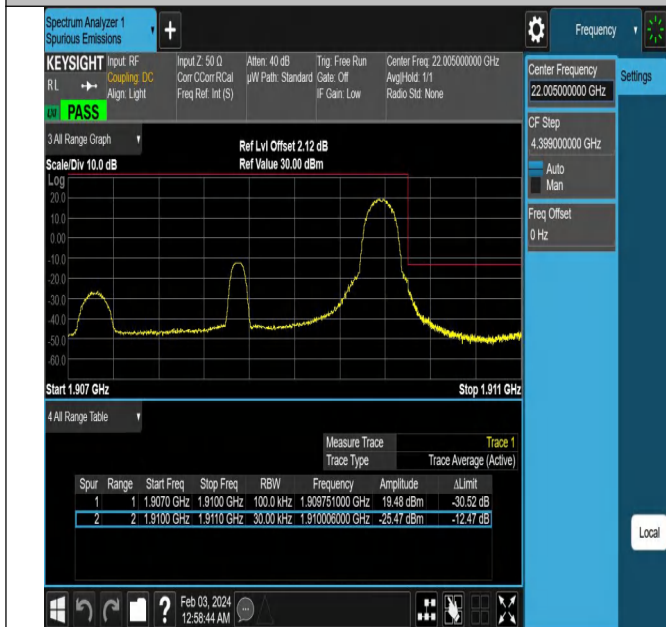
Band2_3MHz_QPSK_19185_1RB#14
