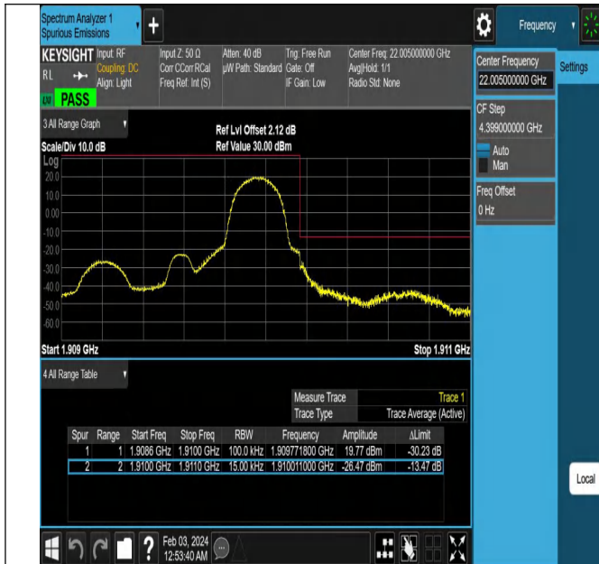
Band2_1.4MHz_QPSK_19193_1RB#5
