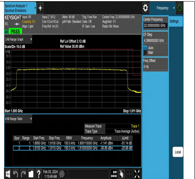
Band2_15MHz_QPSK_19125_75RB#0
