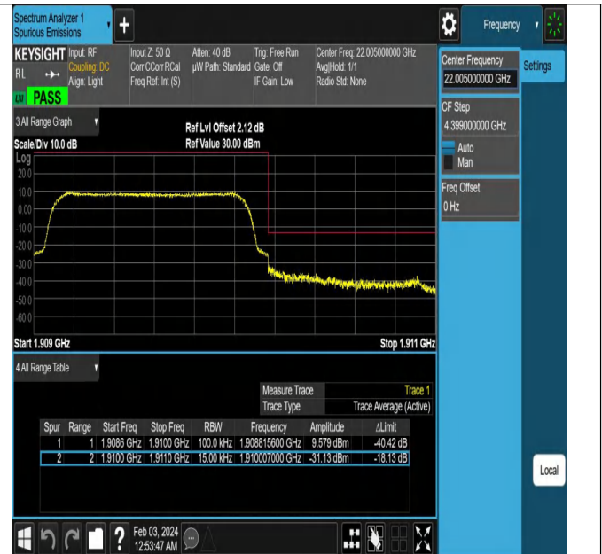
Band2_1.4MHz_QPSK_19193_6RB#0
