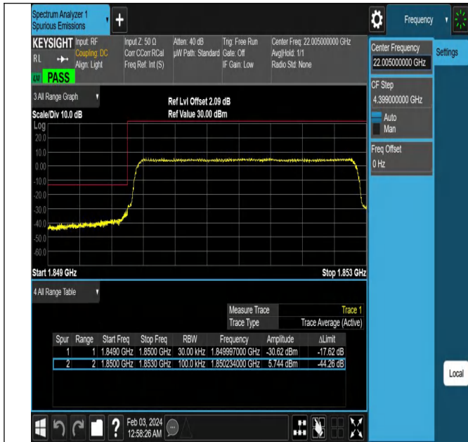
Band2_3MHz_QPSK_18615_15RB#0
