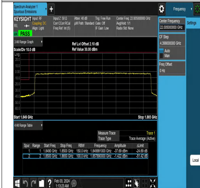
Band2_15MHz_QPSK_18675_75RB#0
