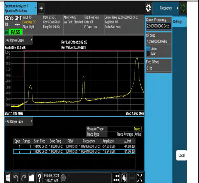
Band2_10MHz_QPSK_18650_1RB#49
