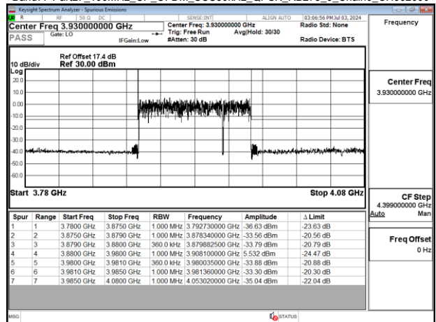
Band77-Part27_100MHz_CP_OFDM_SCS30kHz_QPSK_RB273_0_Chain0_CH662000
