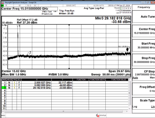
Band41_90MHz_CP_OFDM_SCS30kHz_QPSK_RB1_1_Chain0_CH509004
