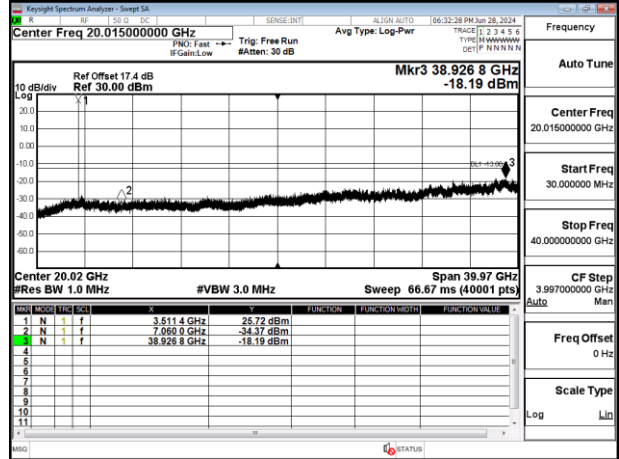
Band77-Part27_40MHz_CP_OFDM_SCS30kHz_QPSK_RB1_1_Chain0_CH648000
