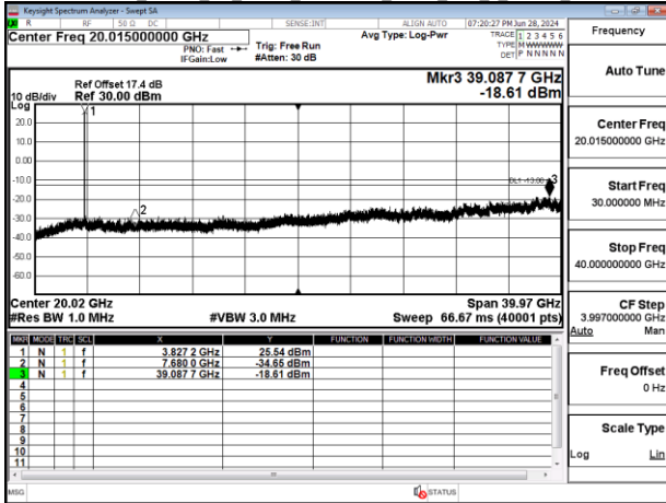
Band77-Part27_30MHz_CP_OFDM_SCS30kHz_QPSK_RB1_1_Chain0_CH664332
