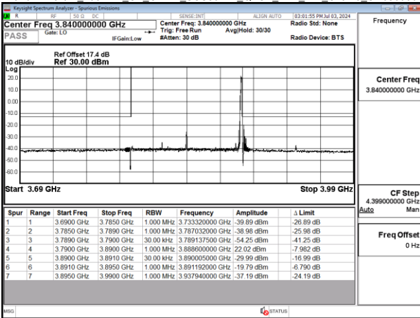
Band77-Part27_100MHz_CP_OFDM_SCS30kHz_QPSK_RB1_272_Chain0_CH662000
