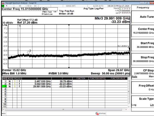
Band41_50MHz_CP_OFDM_SCS30kHz_QPSK_RB1_1_Chain0_CH505002
