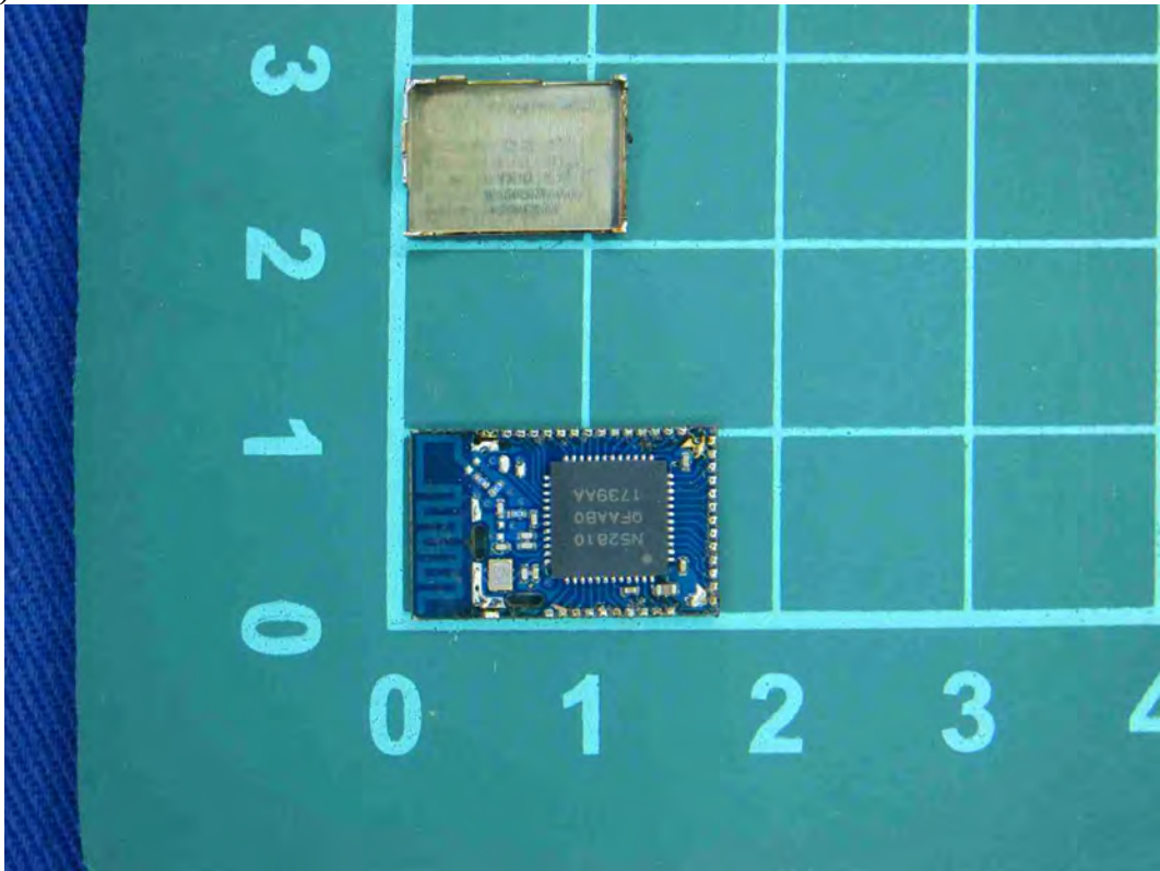
(23) EUT Photo
