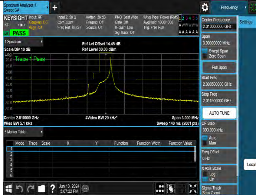
Band23-3.75kHz-MASK-M-BPSK-1@1
