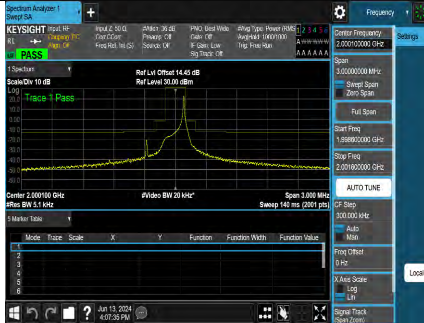
Band23-3.75kHz-MASK-M-QPSK-1@1
