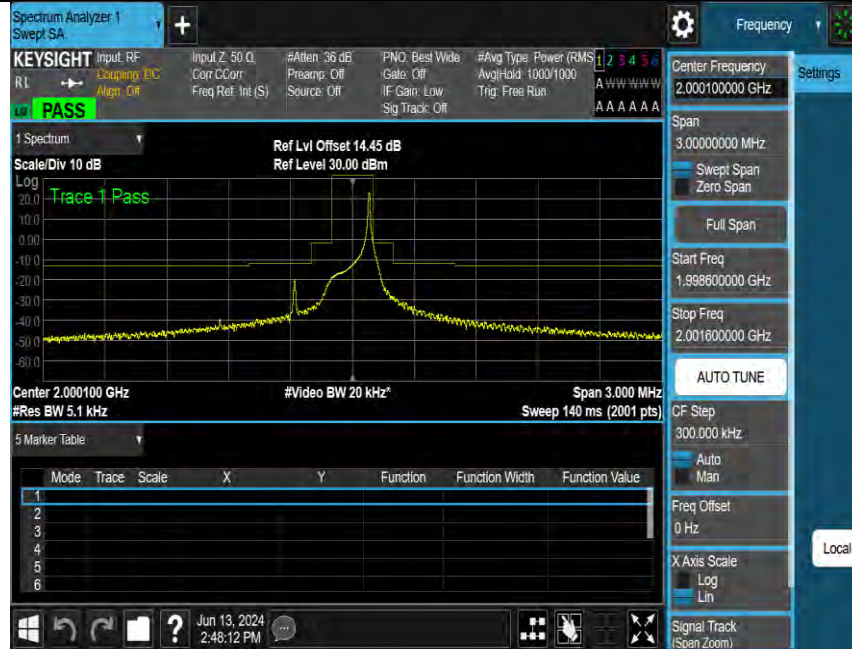
Band23-3.75kHz-MASK-L-BPSK-1@1
