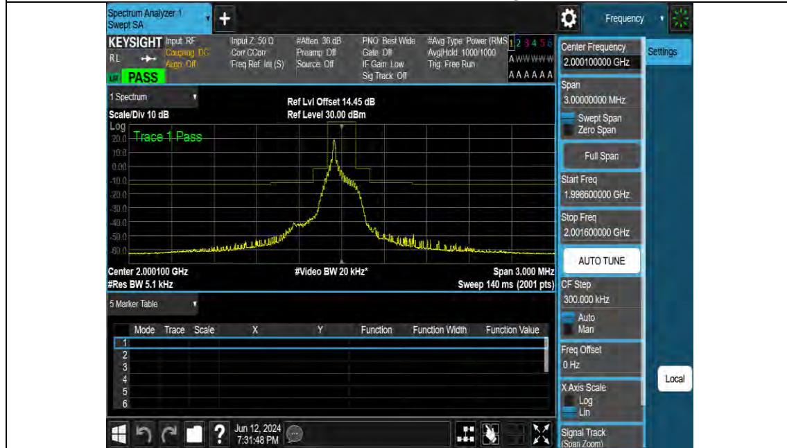
Band23-15kHz-MASK-L-BPSK-1@1
