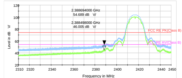
802.11b-Channel 2 Peak & Average
