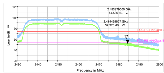
802.11n HT40 -Channel 9 Peak &amp; Average
