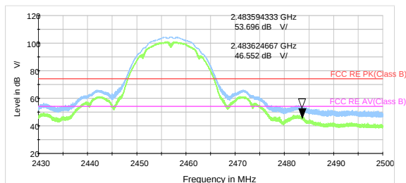
802.11b-Channel 10 Peak & Average
