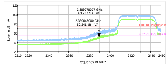
802.11n HT40 -Channel 4 Peak &amp; Average
