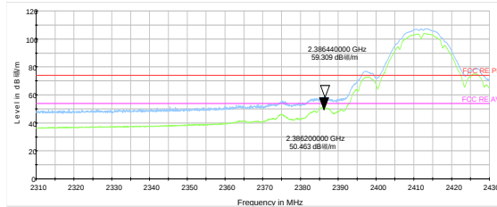
802.11b-Channel 1 Peak & Average
