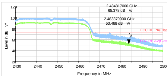
802.11n HT40 -Channel 8 Peak &amp; Average
