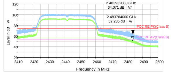
802.11n HT40 -Channel 7 Peak &amp; Average
