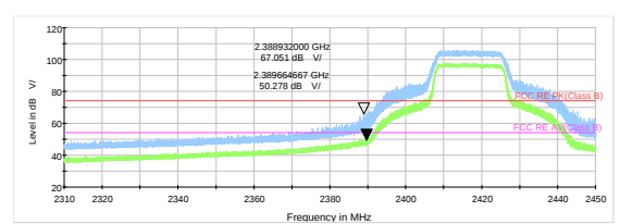
802.11n HT20 -Channel 2 Peak & Average
