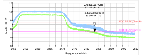
802.11n HT20 -Channel 11 Peak &amp; Average
