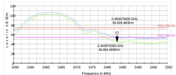
802.11b-Channel 11 Peak & Average
