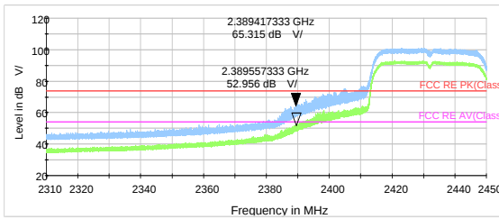
802.11n HT40 -Channel 5 Peak &amp; Average
