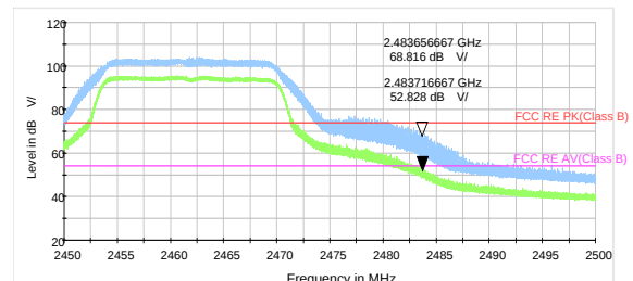
802.11g-Channel 11 Peak & Average
