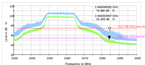
802.11g-Channel 10 Peak & Average
