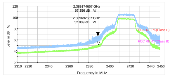
802.11g-Channel 2 Peak & Average
