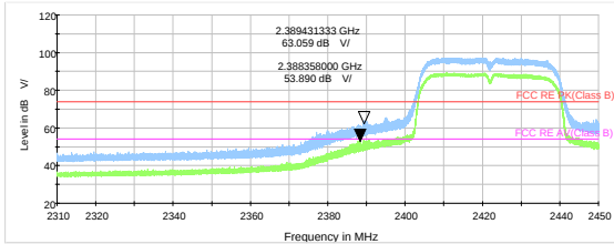
802.11n HT40 -Channel 3 Peak &amp; Average
