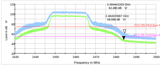
802.11n HT20 -Channel 10 Peak &amp; Average
