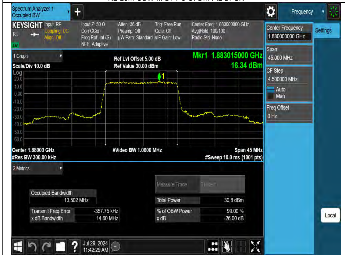
N2-15M-OBW-M-CP-OFDM-QPSK
