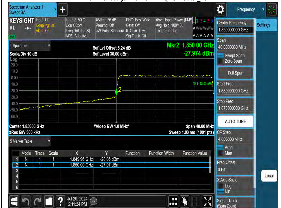
N2-20M-Bandedge-L-CP-OFDM-QPSK-1RB0
