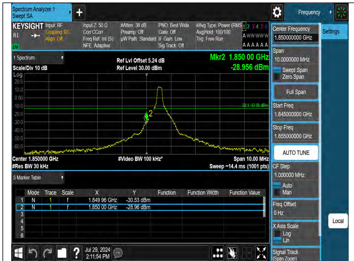
N2-20M-Bandedge-H-DFT-s-OFDM-Pi2 BPSK-Outer Full
