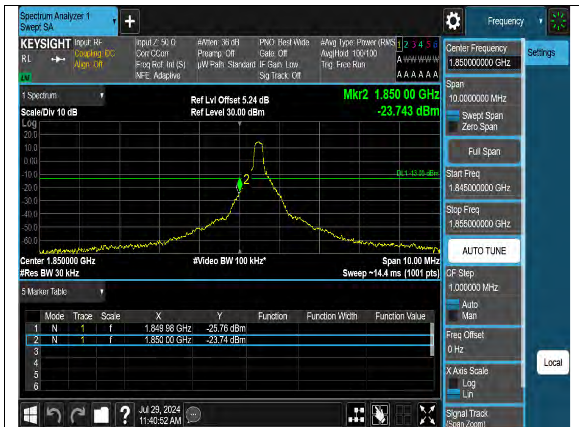
N2-15M-Bandedge-L-CP-OFDM-QPSK-Outer_Full
