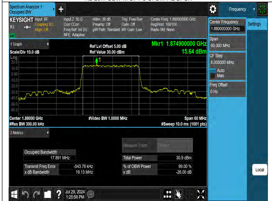
N2-20M-OBW-M-CP-OFDM-QPSK
