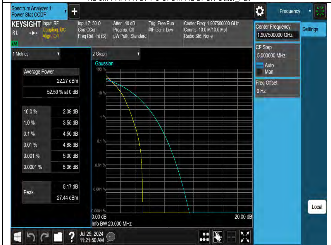
N2-5M-PAPR-H-CP-OFDM-QPSK-Outer Full
