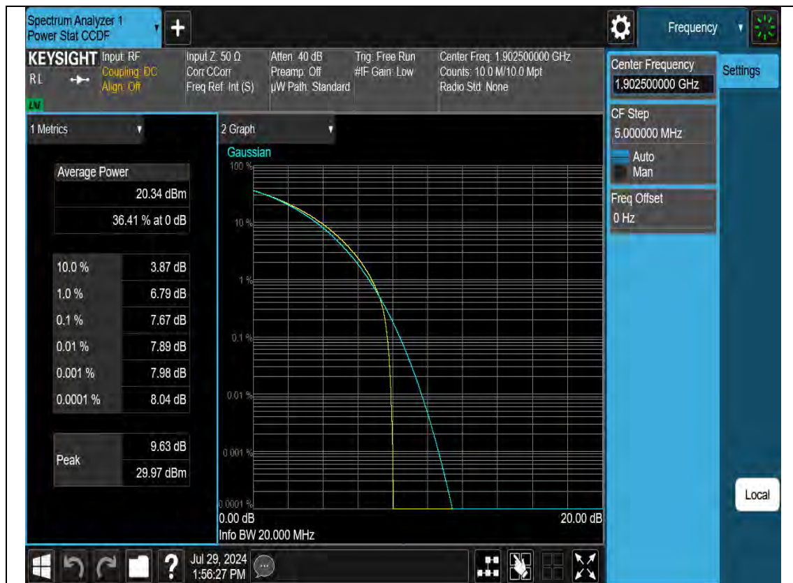
N2-20M-PAPR-L-DFT-s-OFDM-Pi2 BPSK-Outter Full
