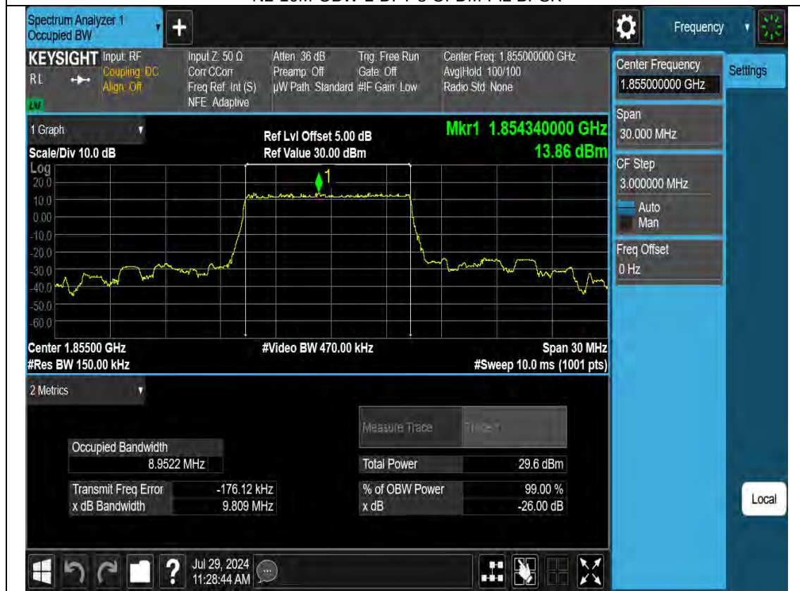
N2-10M-OBW-L-CP-OFDM-QPSK
