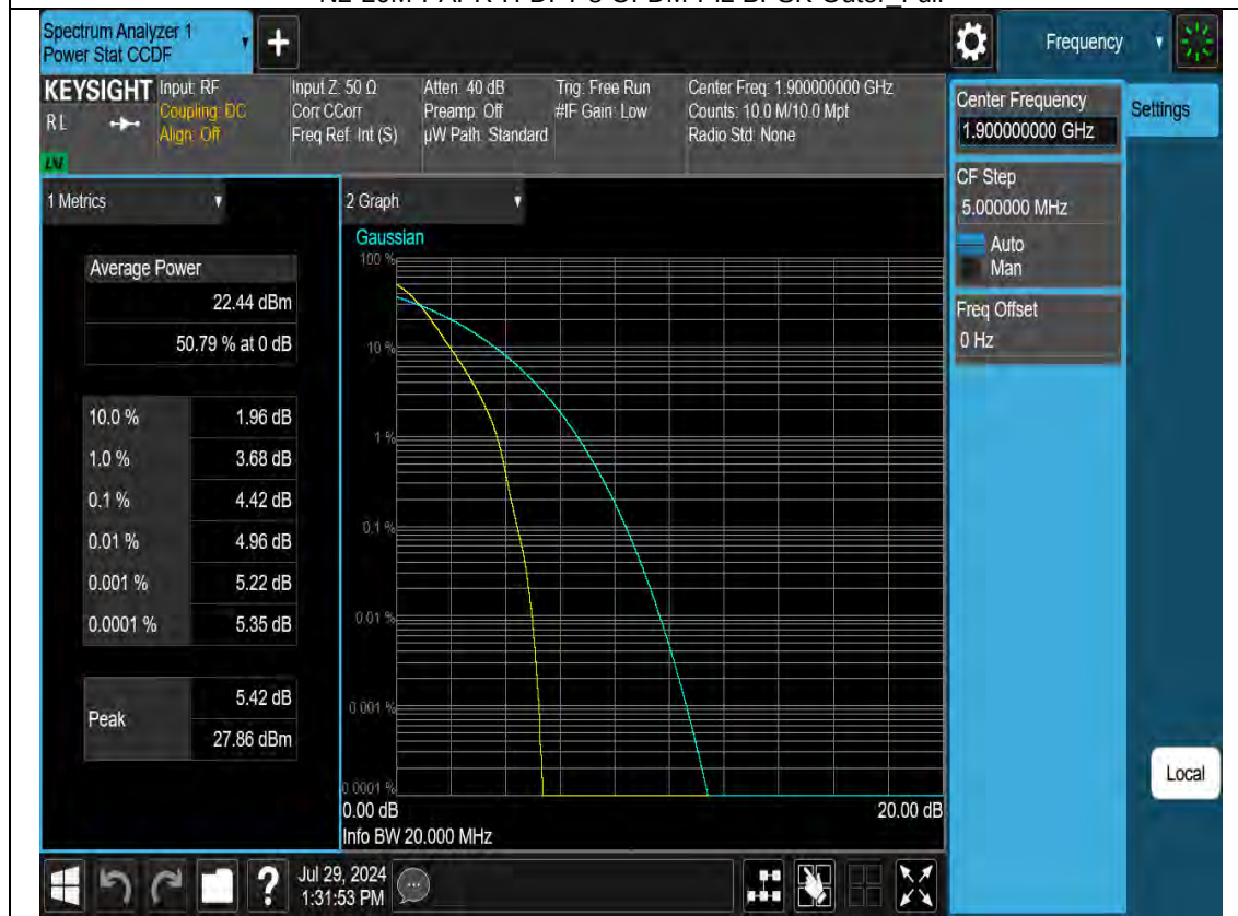
N2-20M-PAPR-H-CP-OFDM-QPSK-Outer Full
