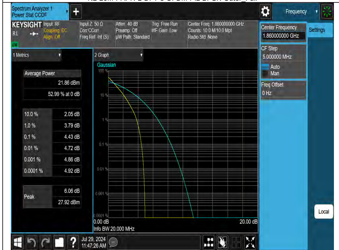
N2-20M-PAPR-L-CP-OFDM-QPSK-Outter Full
