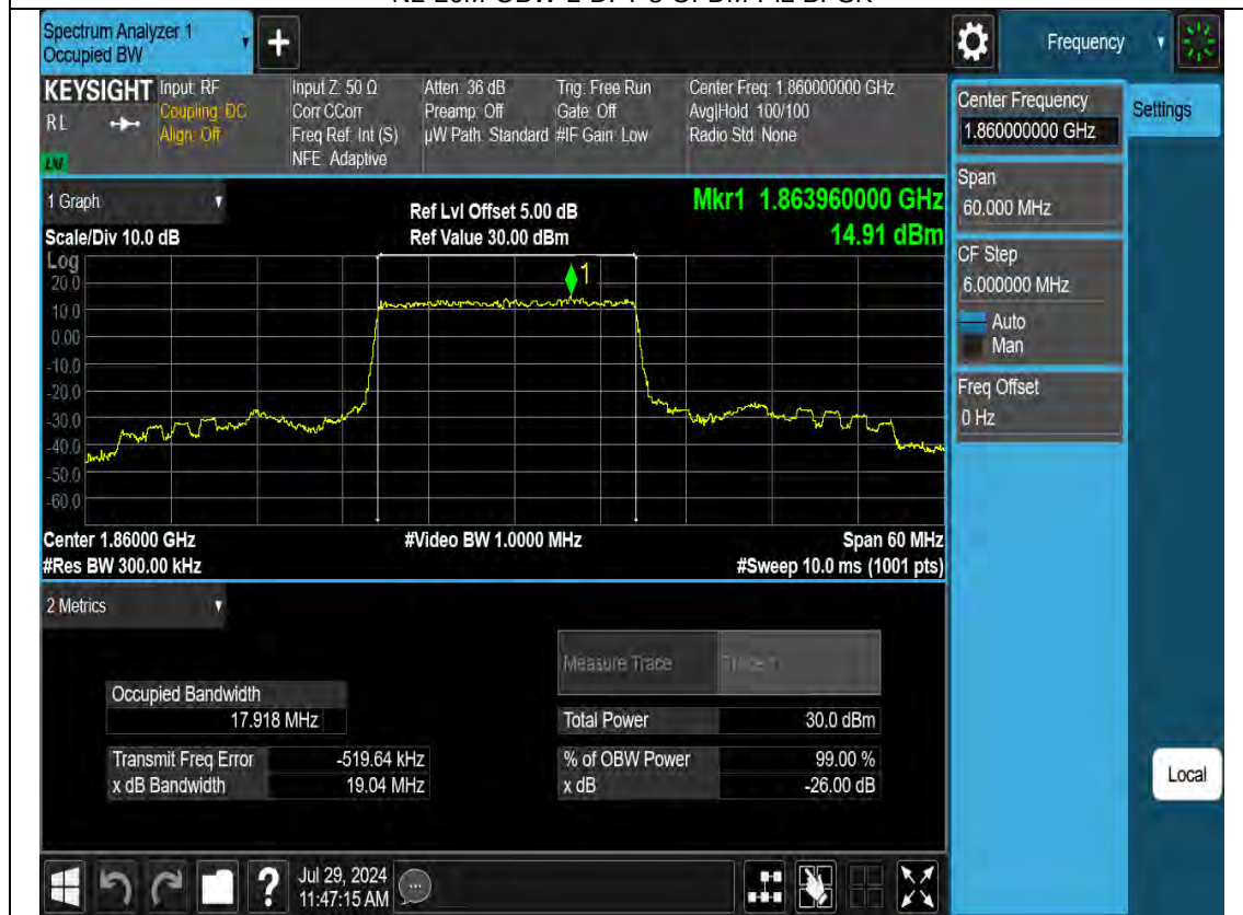
N2-20M-OBW-L-CP-OFDM-QPSK
