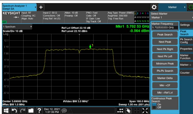
Channel 138 (5690MHz)
