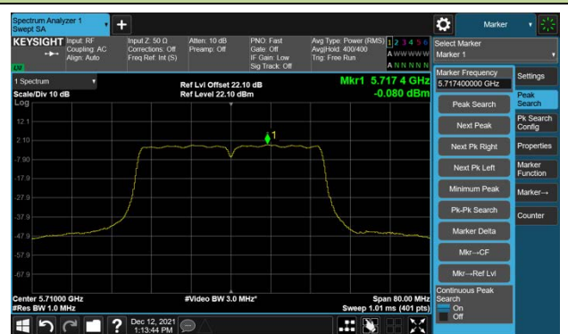
Channel 142 (5710MHz)
