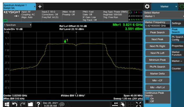
Channel 165 (5825MHz)
