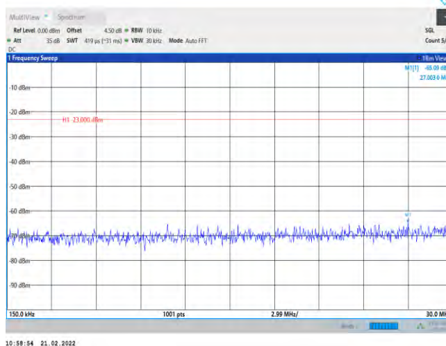
Band26-15MHz-QPSK-26865-1RB#0-Range2:0.15~30MHz
