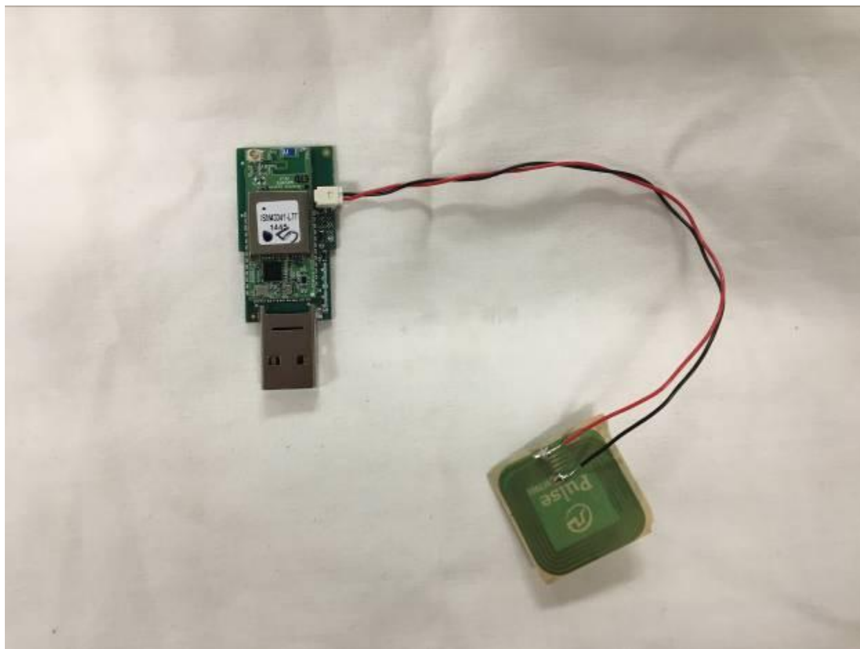
Figure 3. Radio Module on USB Carrier Board (this configuration supports WiFi+BT+NFC)
