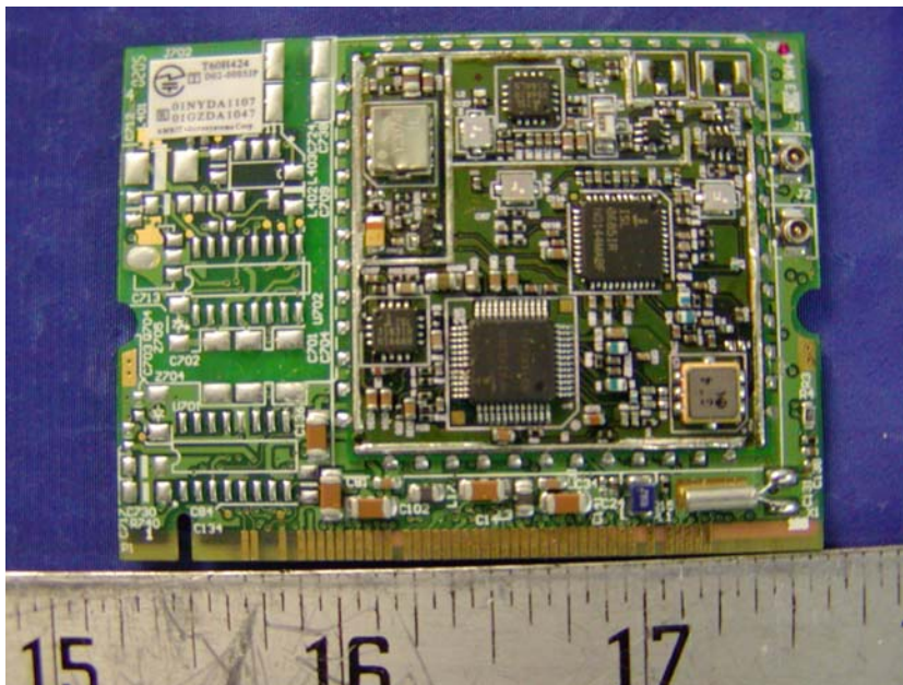
Shield Removed Component View
