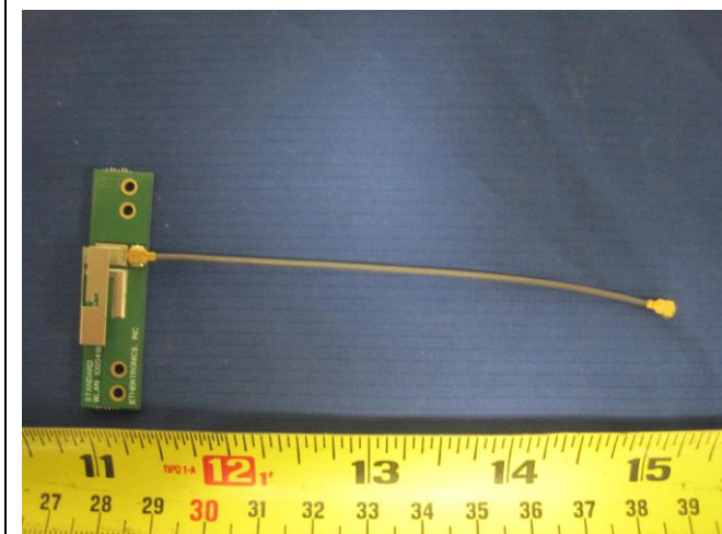
Antenna – Top View (Embedded antenna)
