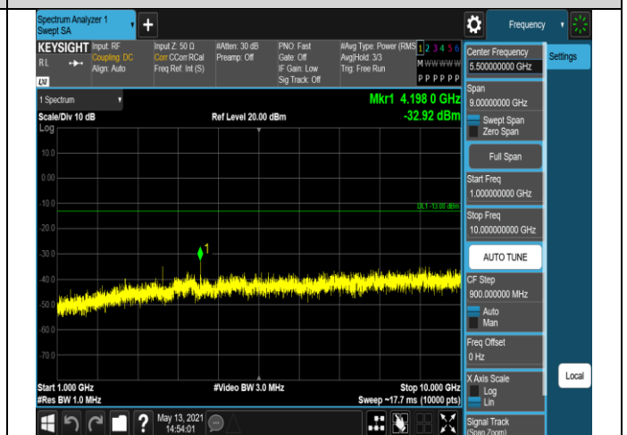
Band5-10MHz-16QAM-20450-1RB#0-Range2:1000~10
