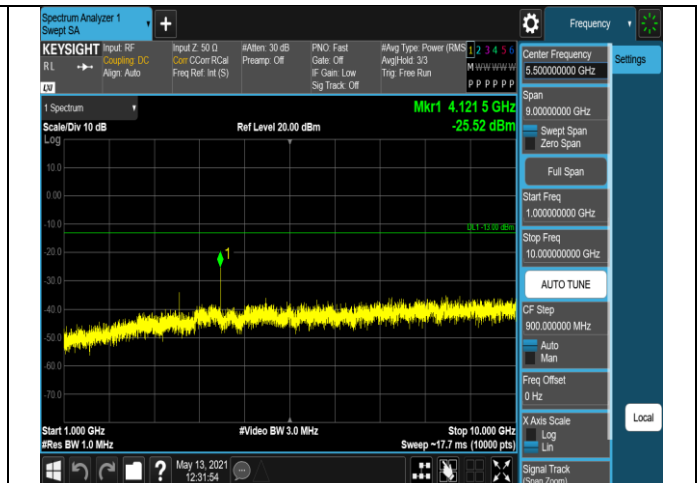
Band5-1.4MHz-QPSK-20525-1RB#0-Range2:1000~10
