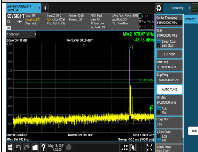
Band5-10MHz-QPSK-20600-1RB#0-Range1:30~10
