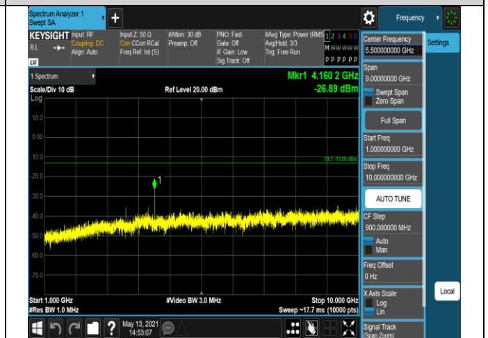
Band5-10MHz-QPSK-20600-1RB#0-Range2:1000~100
