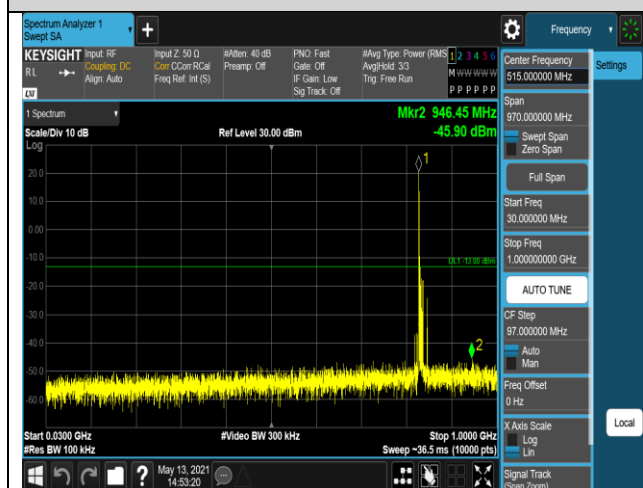
Band5-10MHz-16QAM-20600-1RB#0-Range1:30~1
