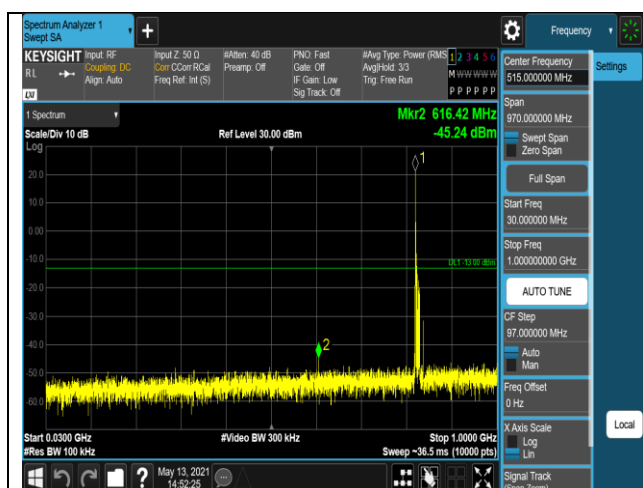
Band5-10MHz-16QAM-20525-1RB#0-Range1:30~1
