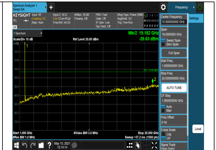
Band4-20MHz-16QAM-20175-1RB#0-Range2:1000~20
