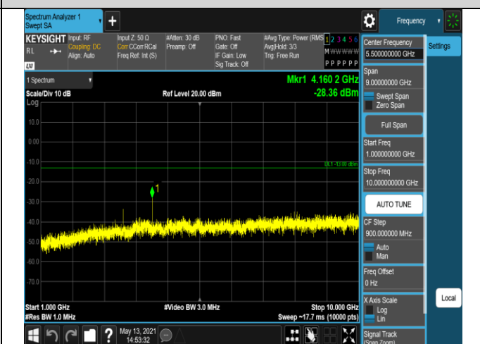
Band5-10MHz-16QAM-20600-1RB#0-Range2:1000~10
