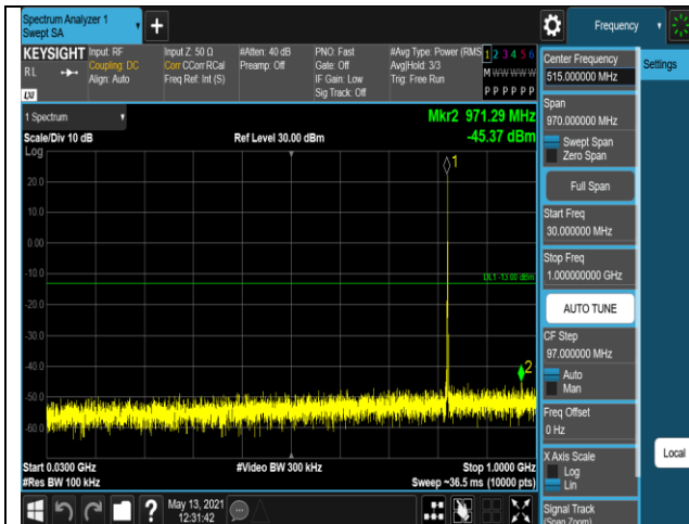
Band5-1.4MHz-QPSK-20525-1RB#0-Range1:30~10
