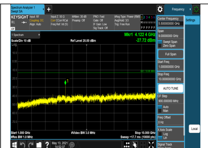
Band5-10MHz-16QAM-20525-1RB#0-Range2:1000~10
