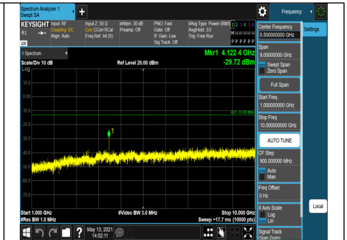
Band5-10MHz-QPSK-20525-1RB#0-Range2:1000~100
