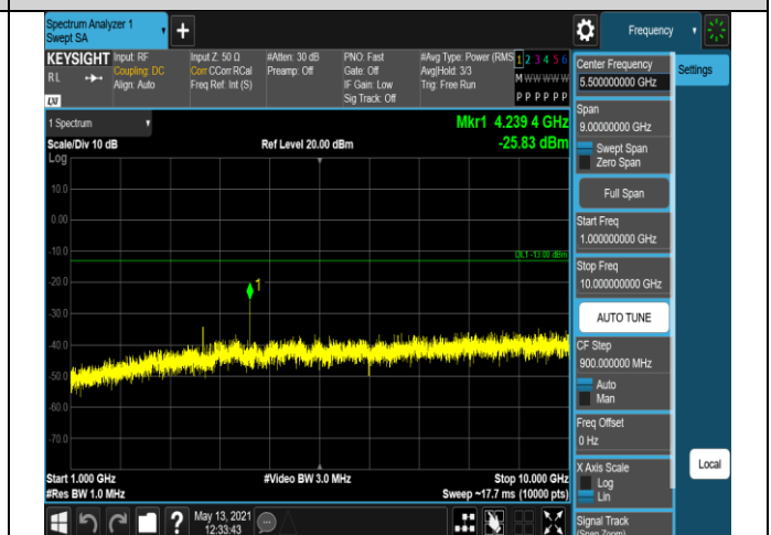
Band5-1.4MHz-16QAM-20407-1RB#0-Range2:1000~1
