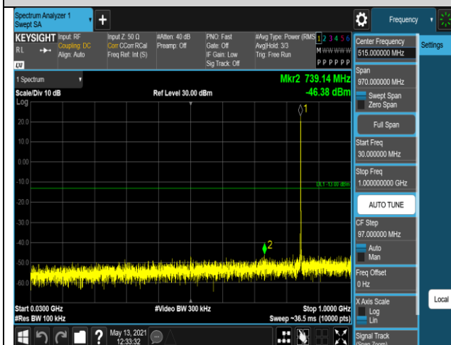
Band5-1.4MHz-16QAM-20407-1RB#0-Range1:30~1
