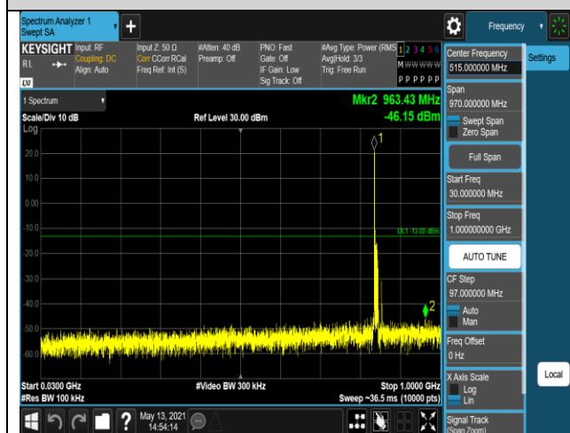
Band12-1.4MHz-QPSK-23017-1RB#0-Range1:30~1
