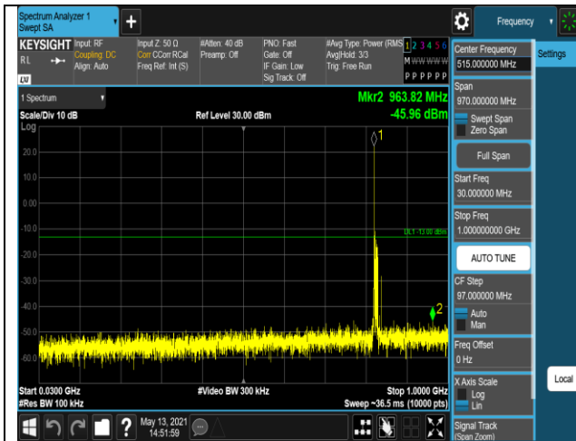
Band5-10MHz-QPSK-20525-1RB#0-Range1:30~10
