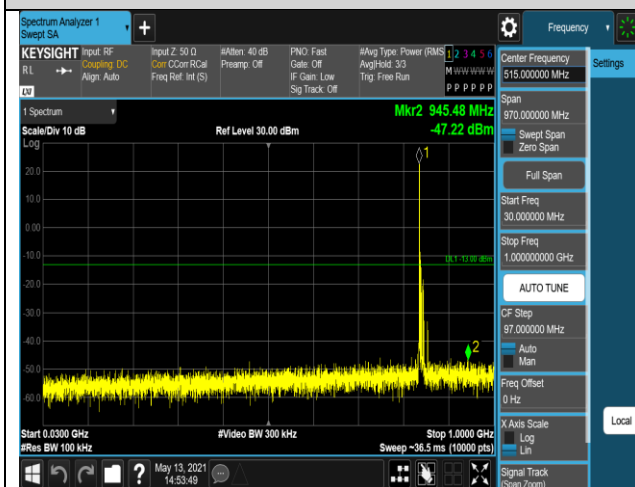
Band5-10MHz-16QAM-20450-1RB#0-Range1:30~1
