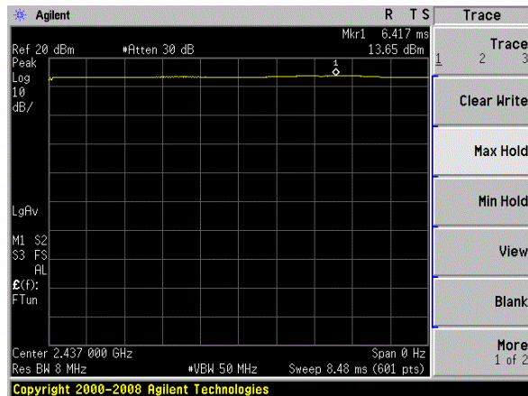
(802.11n20) channel 6
