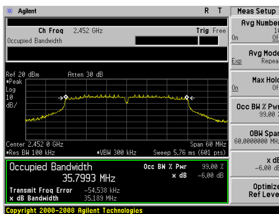
(802.11n40) 6dB Bandwidth plot on channel 9
