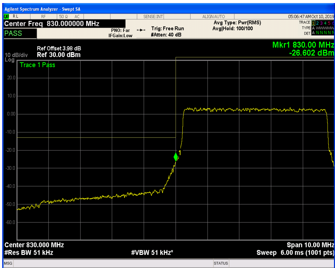
LTE Band19 QAM16 BW=5MHz Channel=24025 RB Size=25 Position=#0
