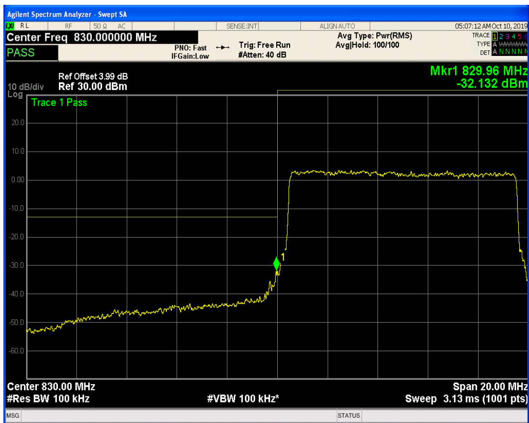
LTE Band19 QAM16 BW=10MHz Channel=24050 RB Size=50 Position=#0
