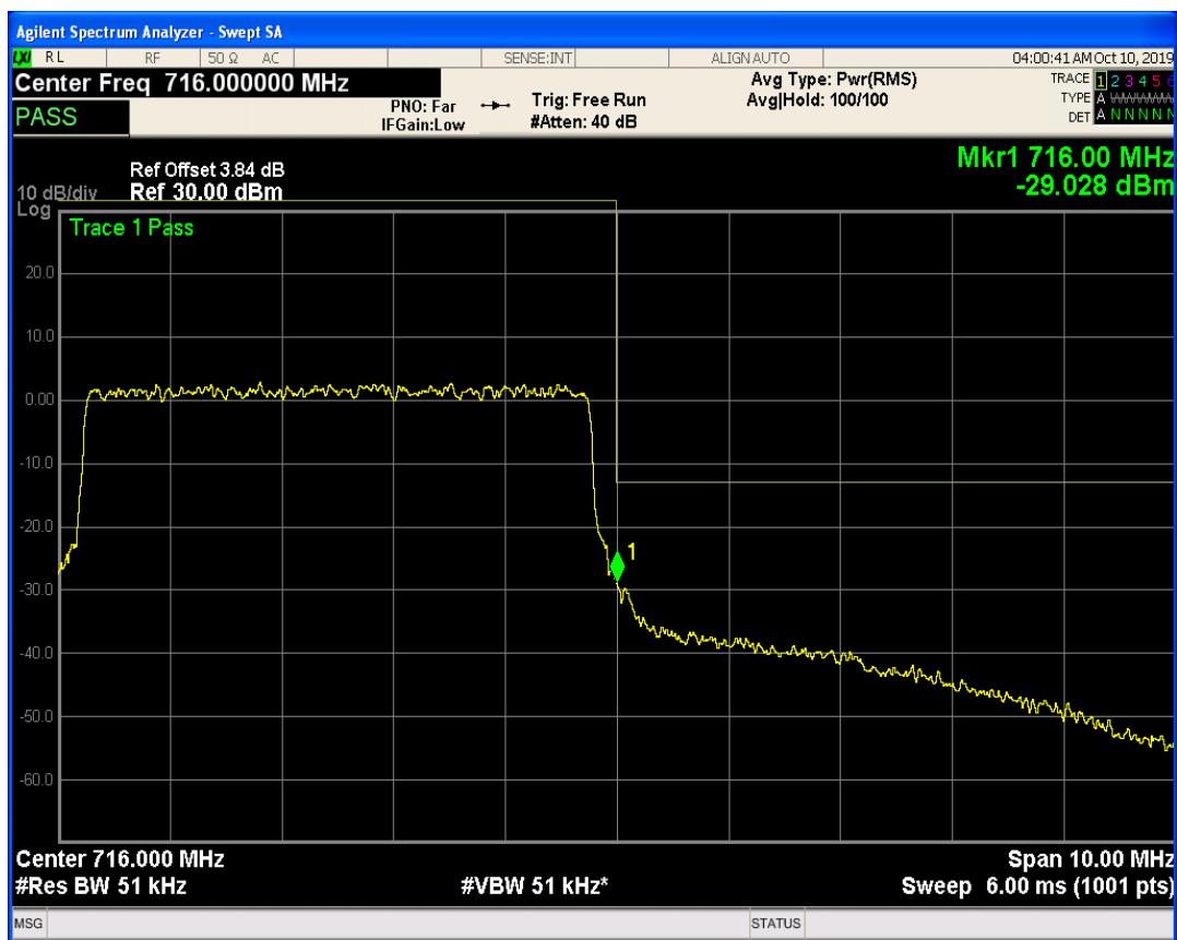
LTE Band17 QAM16 BW=5MHz Channel=23825 RB Size=1 Position=#Max
