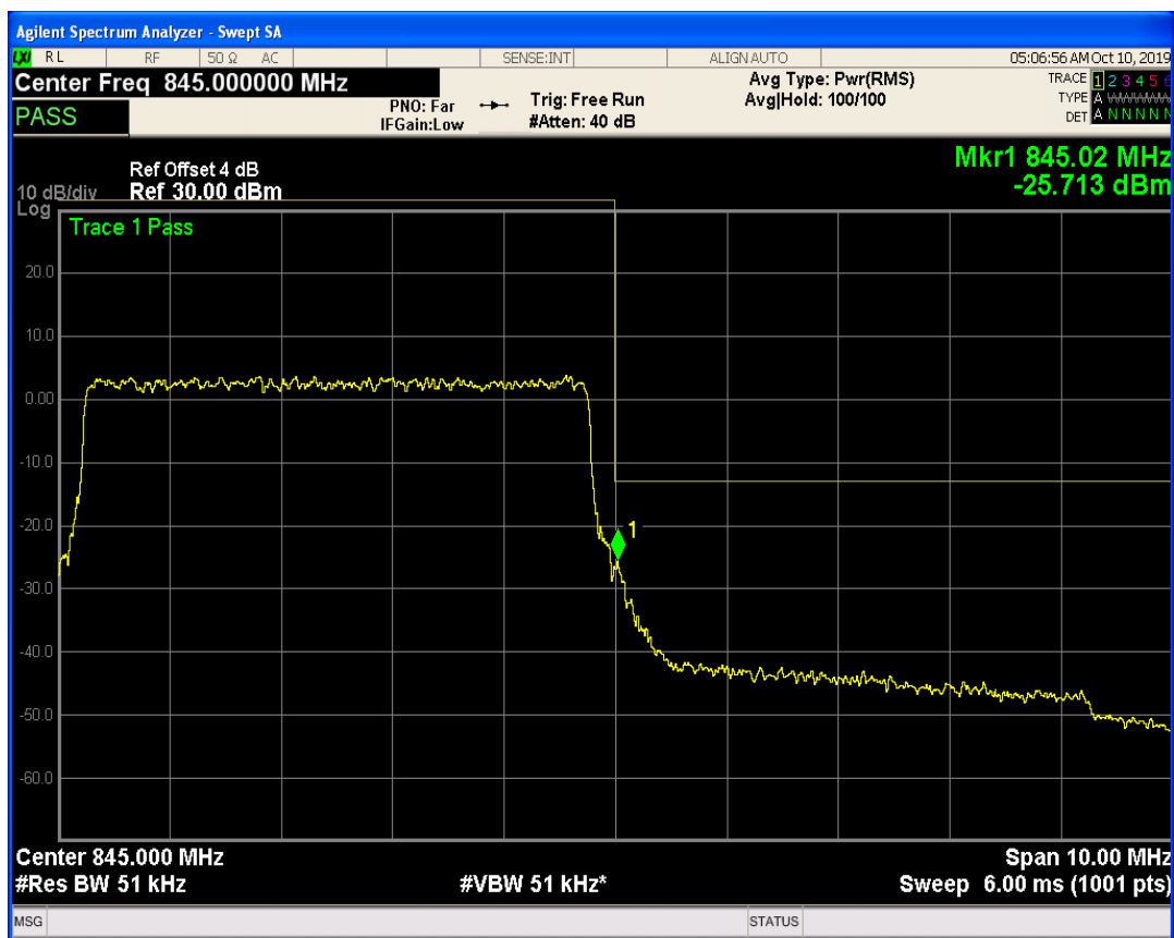
LTE Band19 QAM16 BW=5MHz Channel=24125 RB Size=25 Position=#0
