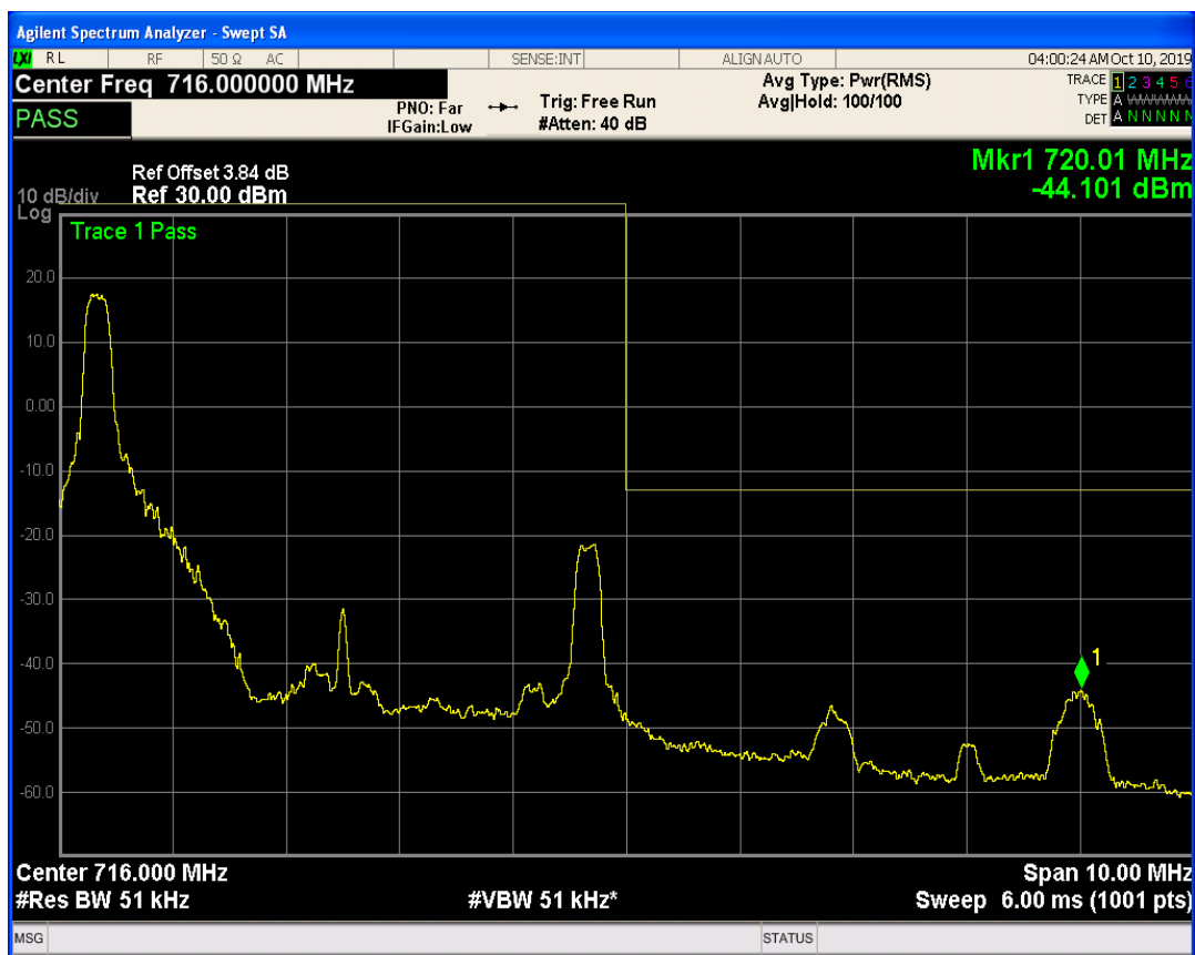
LTE Band17 QPSK BW=5MHz Channel=23825 RB Size=1 Position=#Max
