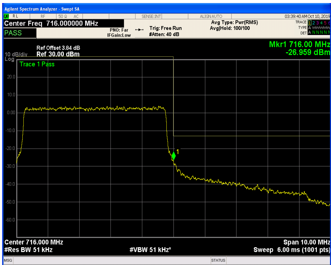
LTE Band12 QAM16 BW=5MHz Channel=23155 RB Size=1 Position=#Max
