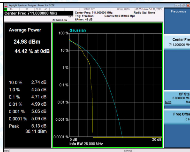
Band12-10MHz-QPSK-23130-1RB#0-PASS
