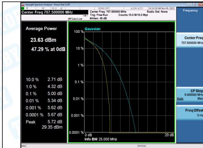
Band12-1.4MHz-QPSK-23095-6RB#0-PASS
