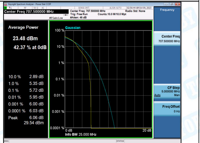
Band12-5MHz-16QAM-23095-1RB#0-PASS
