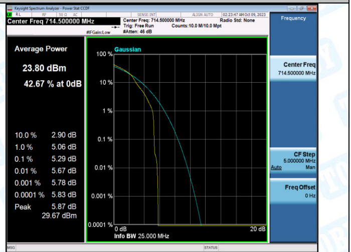
Band12-3MHz-16QAM-23165-1RB#0-PASS
