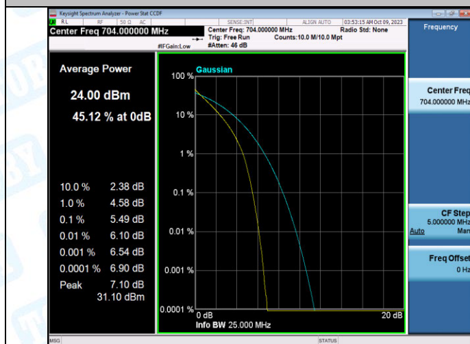
Band12-10MHz-QPSK-23060-50RB#0-PASS
