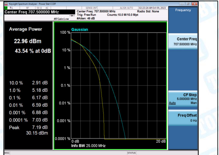
Band12-3MHz-16QAM-23095-15RB#0-PASS
