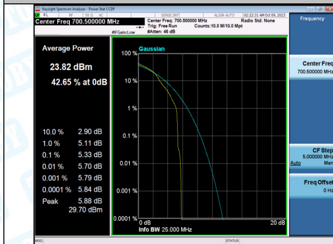
Band12-3MHz-16QAM-23025-1RB#0-PASS
