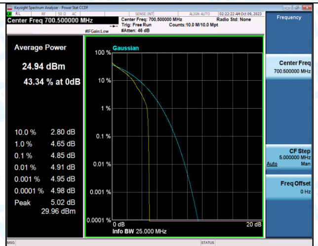
Band12-3MHz-QPSK-23025-1RB#0-PASS
