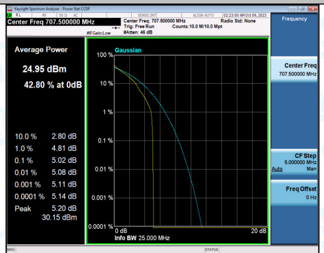
Band12-3MHz-QPSK-23095-1RB#0-PASS
