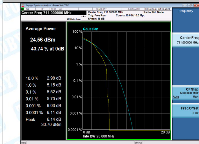
Band12-10MHz-16QAM-23130-1RB#0-PASS
