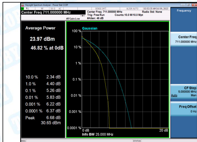
Band12-10MHz-QPSK-23130-50RB#0-PASS
