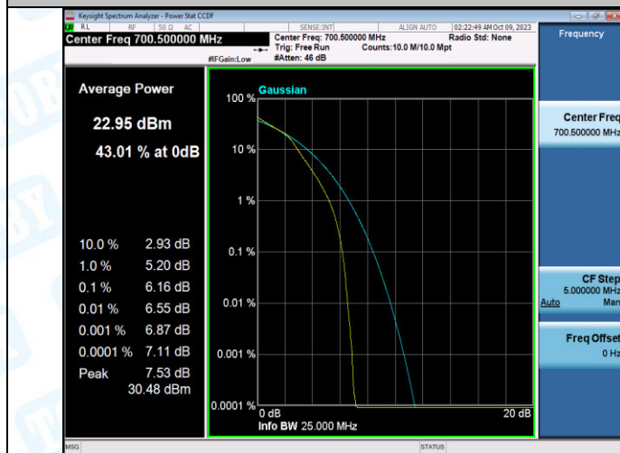
Band12-3MHz-16QAM-23025-15RB#0-PASS
