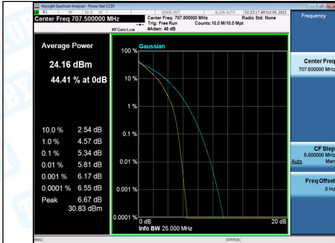
Band12-3MHz-QPSK-23095-15RB#0-PASS
