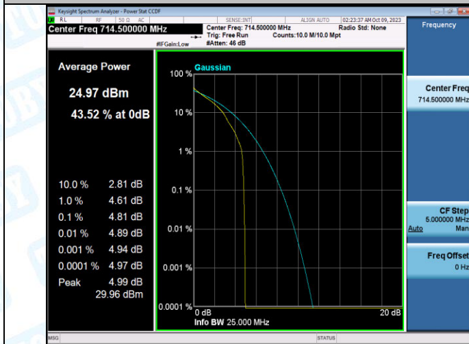
Band12-3MHz-QPSK-23165-1RB#0-PASS
