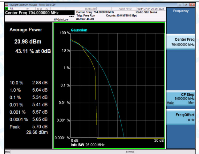
Band12-10MHz-16QAM-23060-1RB#0-PASS
