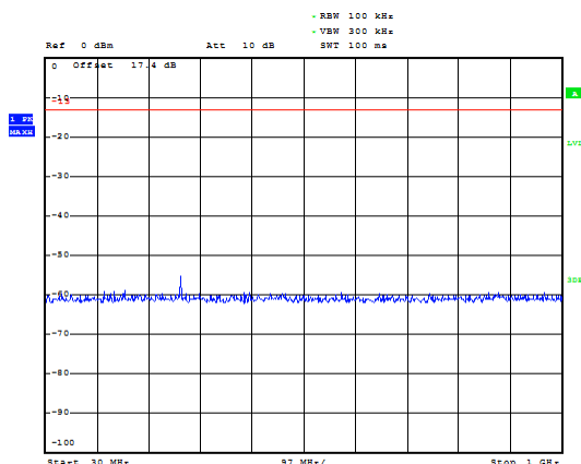
LTE Band 4 1.4MHz CH-Middle 30MHz~1GHz
