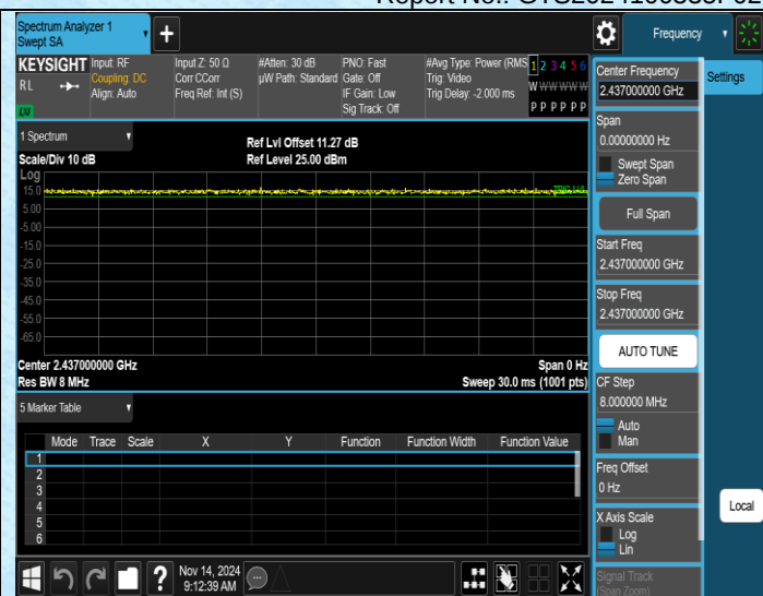
NTNV-11N20SISO-Ant1-2437
