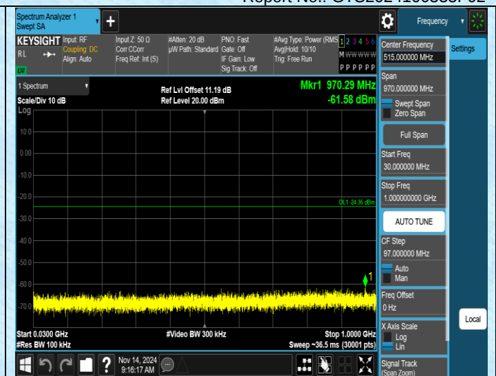
11N20SISO-Ant1-2462-30~1000-PASS
