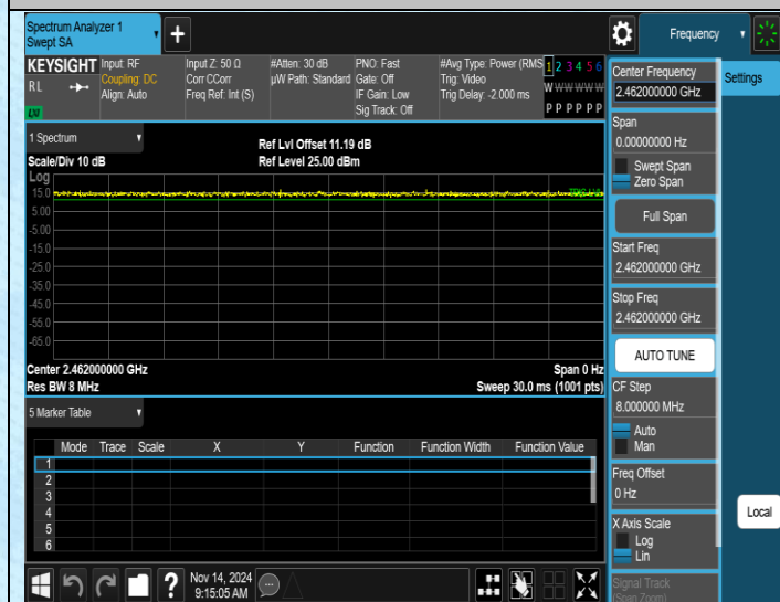
NTNV-11N20SISO-Ant1-2462
