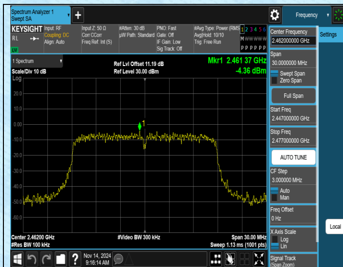
11N20SISO-Ant1-2462-0~Reference-PASS
