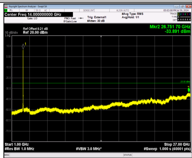
41-41-20MHz-10MHz-64QAM-64QAM-41391-41535-100RB #0-50RB#0-1000~27000MHz-PASS
