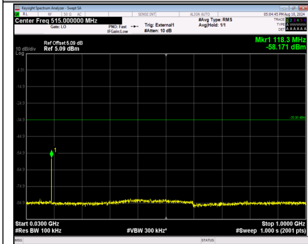
41-41-20MHz-10MHz-16QAM-16QAM-41391-41535-1RB #99-ORB#0-30~1000MHz-PASS
