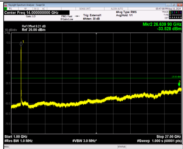
41-41-20MHz-20MHz-QPSK-QPSK-39750-39948-100RB#0 -100RB#0-1000~27000MHz-PASS
