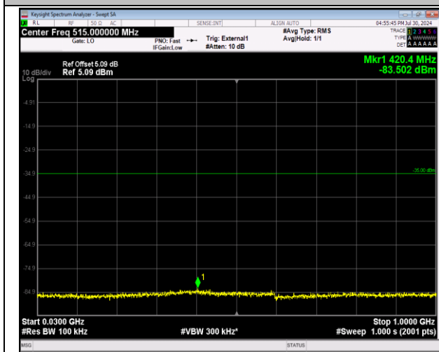
41-41-20MHz-10MHz-64QAM-64QAM-39750-39894-100RB RB#0-50RB#0-30~1000MHz-PASS
