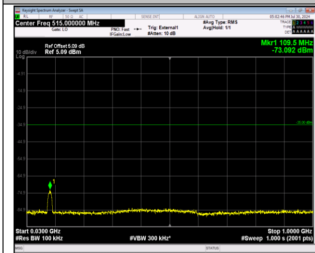
41-41-20MHz-10MHz-64QAM-64QAM-41391-41535-100RB RB#0-50RB#0-30~1000MHz-PASS
