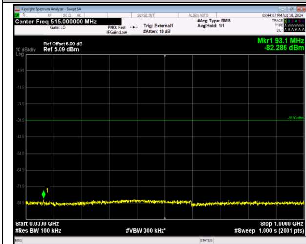
41-41-20MHz-20MHz-16QAM-16QAM-39750-39948-1RB #99-ORB#0-30~1000MHz-PASS
