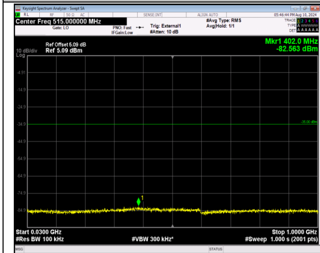
41-41-20MHz-20MHz-QPSK-QPSK-39750-39948-100RB #0-100RB#0-30~1000MHz-PASS
