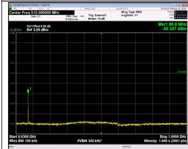
41-41-20MHz-10MHz-QPSK-QPSK-41391-41535-1RB#0 -0RB#0-30~1000MHz-PASS
