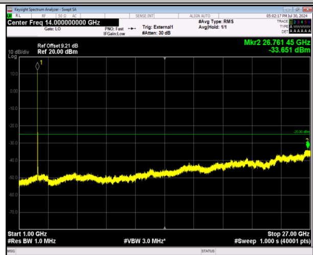
41-41-20MHz-10MHz-64QAM-64QAM-41391-41535-1RB#0 -1RB#49-1000~27000MHz-PASS
