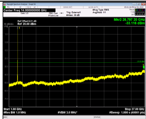
41-41-20MHz-10MHz-64QAM-64QAM-41391-41535-1RB#9 9-0RB#0-1000~27000MHz-PASS
