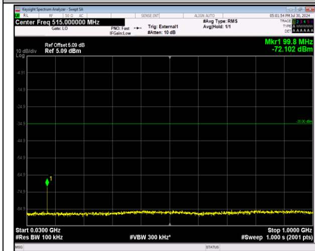
41-41-20MHz-10MHz-64QAM-64QAM-41391-41535-1RB #0-1RB#49-30~1000MHz-PASS
