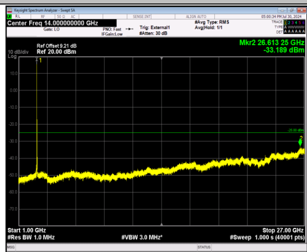
41-41-20MHz-10MHz-64QAM-64QAM-41391-41535-1RB#0 -0RB#0-1000~27000MHz-PASS
