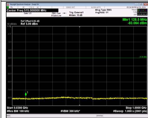
41-41-20MHz-20MHz-64QAM-64QAM-39750-39948-1RB #0-0RB#0-30~1000MHz-PASS
