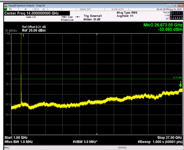
41-41-20MHz-20MHz-16QAM-16QAM-39750-39948-1RB#9 9-ORB#0-1000~27000MHz-PASS
