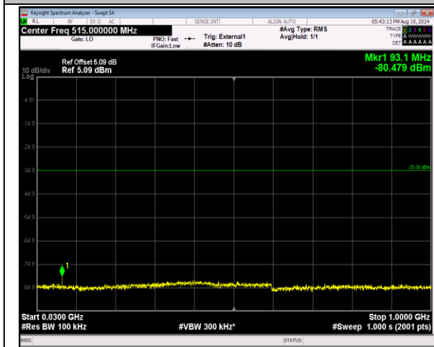
41-41-20MHz-20MHz-QPSK-QPSK-39750-39948-1RB#9 9-0RB#0-30~1000MHz-PASS
