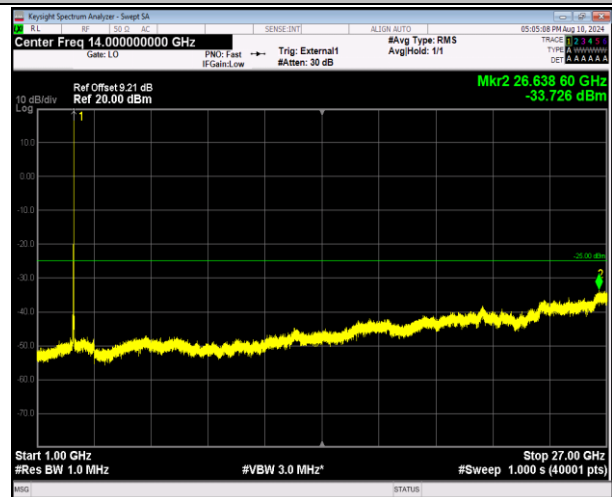
41-41-20MHz-10MHz-16QAM-16QAM-41391-41535-1RB#9 9-ORB#0-1000~27000MHz-PASS
