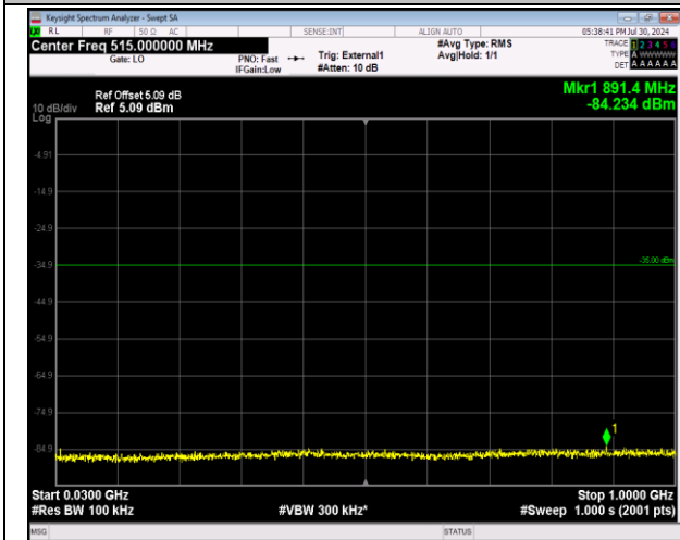
41-41-20MHz-20MHz-64QAM-64QAM-39750-39948-1RB #0-1RB#99-30~1000MHz-PASS
