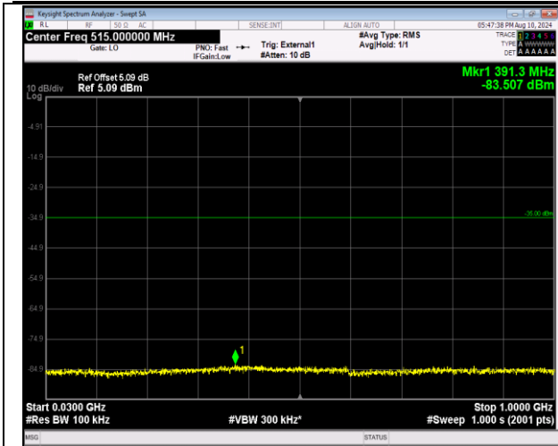
41-41-20MHz-20MHz-16QAM-16QAM-39750-39948-100 RB#0-100RB#0-30~1000MHz-PASS
