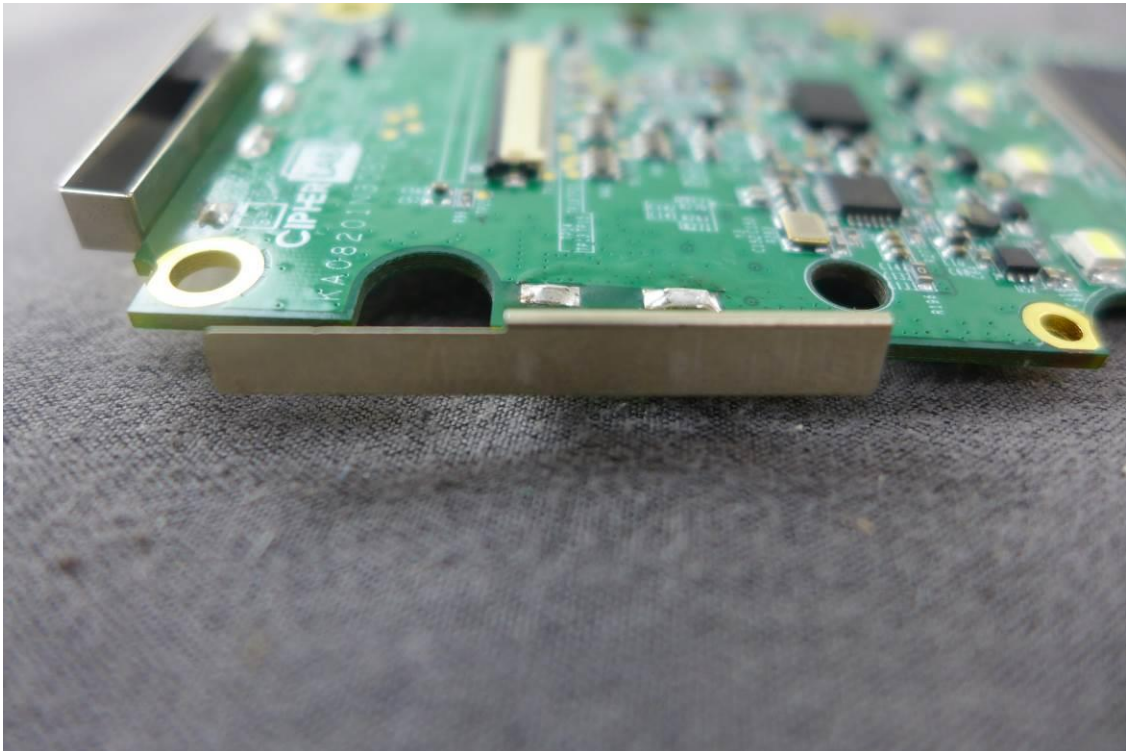
BT Antenna
