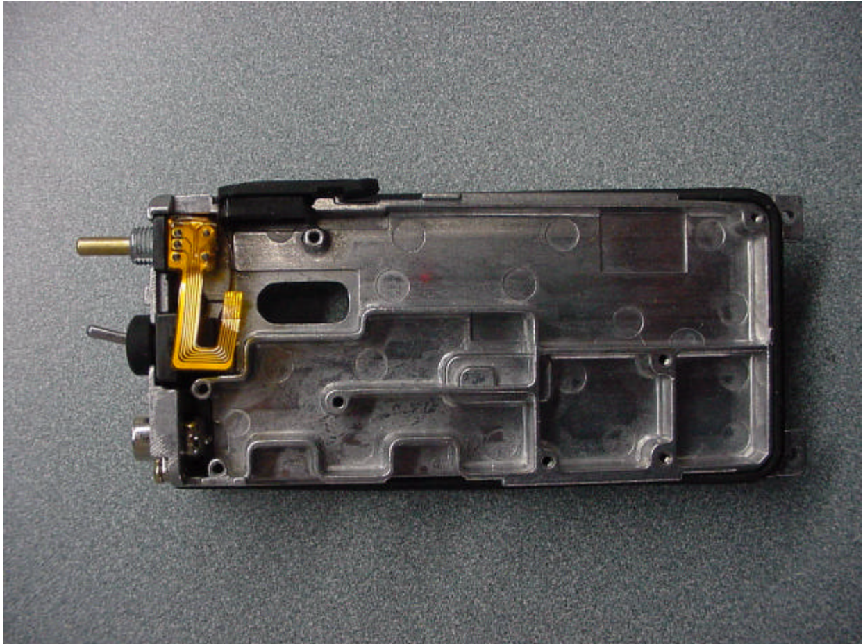
PHOTOGRAPH 11: INSIDE BACK CHASSIS (MURS-22)
