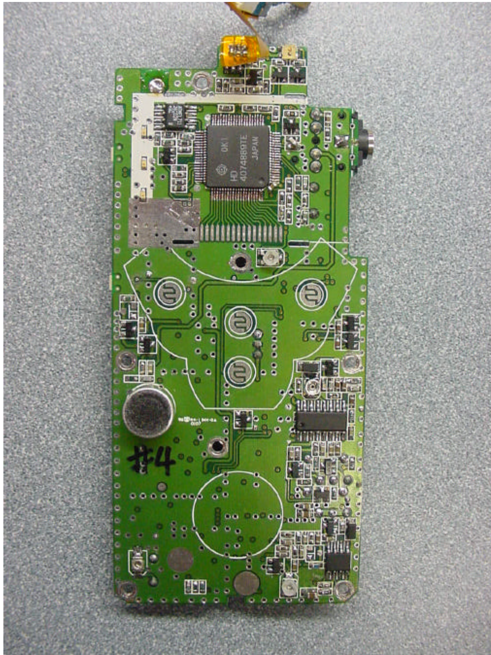
PHOTOGRAPH 18: FRONT OF PCB WITH LCD REMOVED (MURS-25)
