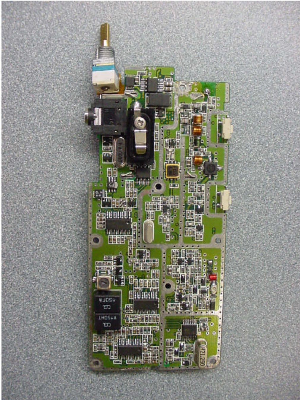
PHOTOGRAPH 15: BACK OF PCB (MURS-25)
