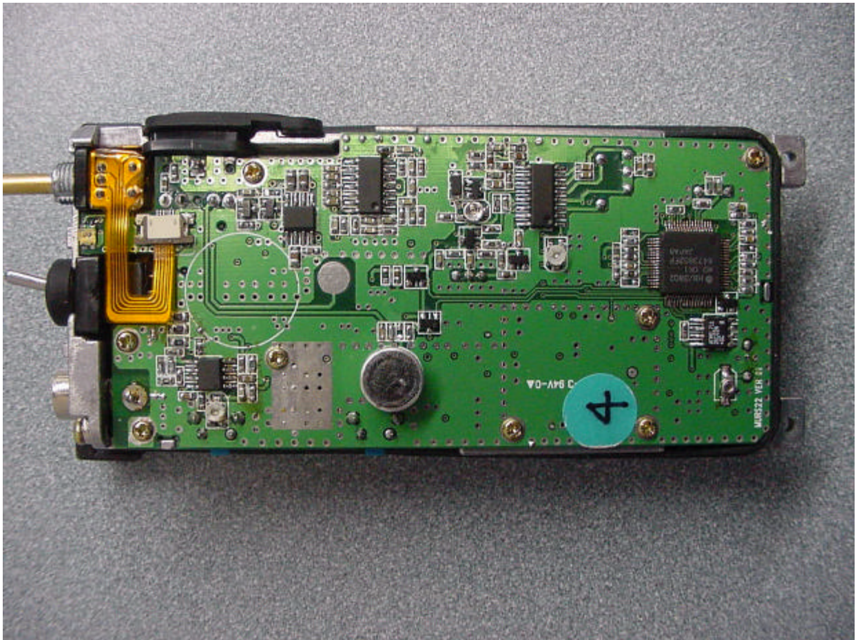
PHOTOGRAPH 9: PCB FRONT IN CHASSIS (MURS-22)
