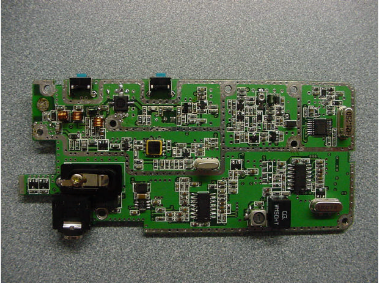
PHOTOGRAPH 7: PCB FRONT (MURS-22)
