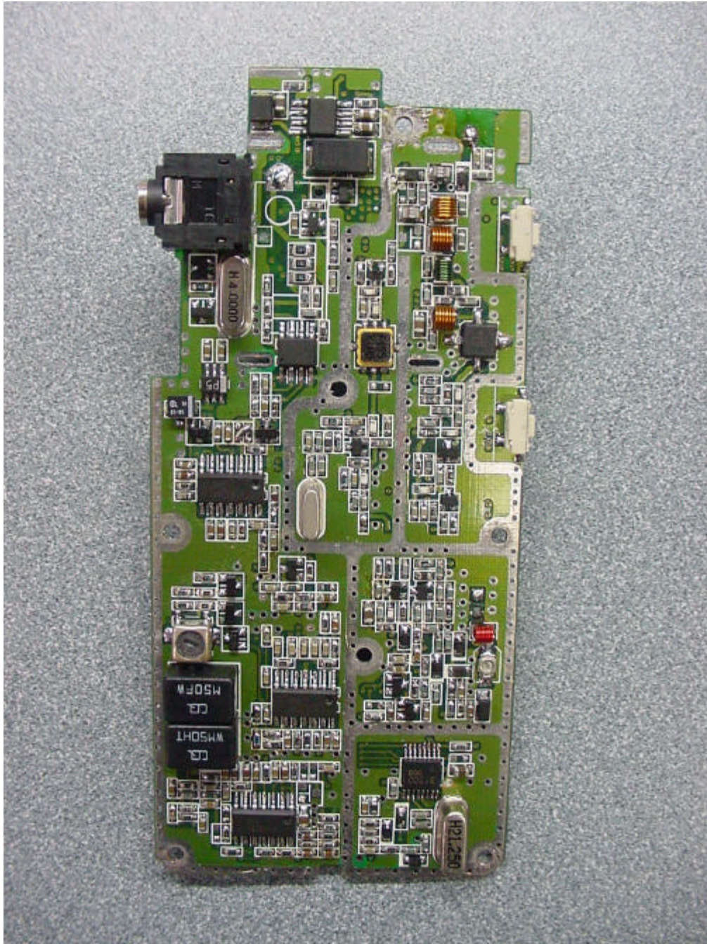
PHOTOGRAPH 16:BACK OF PCB WITH POSITIVE BATTERY TERMINAL REMOVED (MURS-25)
