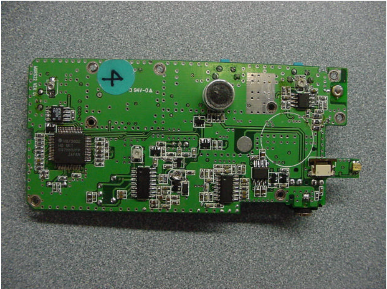
PHOTOGRAPH 8: PCB BACK (MURS-22)
