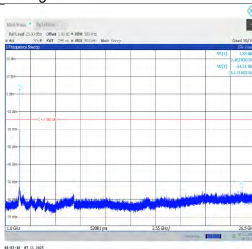
11g-Ant2-2462-1000~26500-PASS
