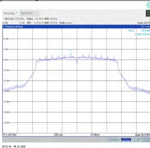
11g-Ant2-2437-0~Reference-PASS
