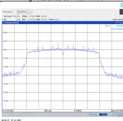
11n20SISO-Ant2-2412-0~Reference-PASS
