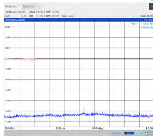
11b-Ant2-2462-30~1000-PASS
