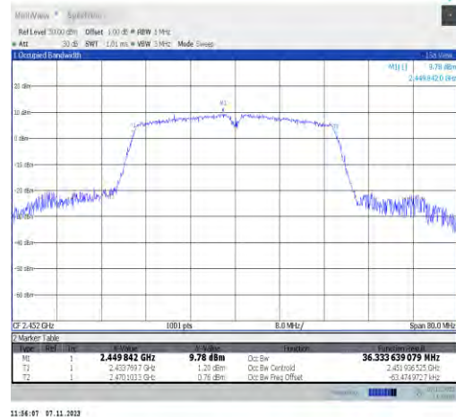
11n40SISO-Ant2-2452
