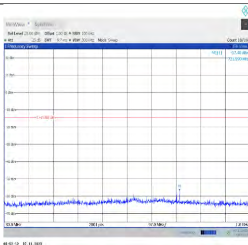
11g-Ant2-2462-30~1000-PASS
