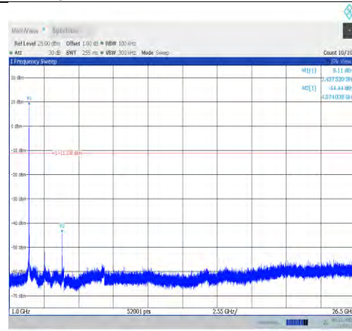
11b-Ant2-2437-1000~26500-PASS
