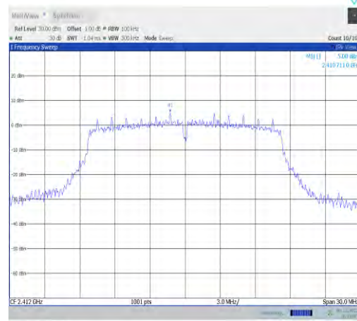
11g-Ant2-2412-0~Reference-PASS
