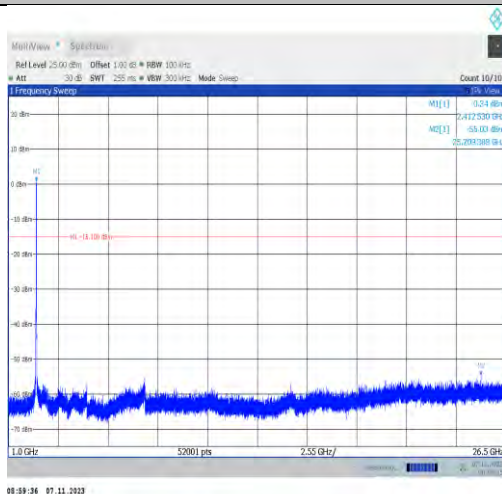
11n20SISO-Ant2-2412-1000~26500-PASS
