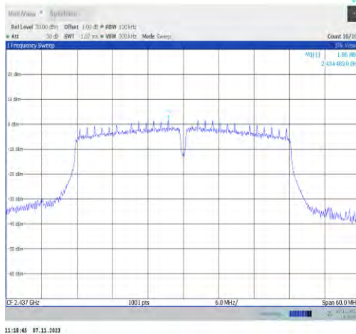
11n40SISO-Ant2-2437-0~Reference-PASS
