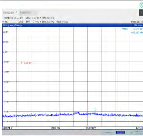
11b-Ant2-2437-30~1000-PASS
