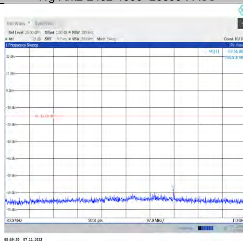
11n20SISO-Ant2-2412-30~1000-PASS
