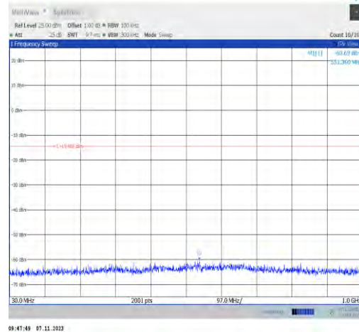
11n20SISO-Ant2-2462-30~1000-PASS
