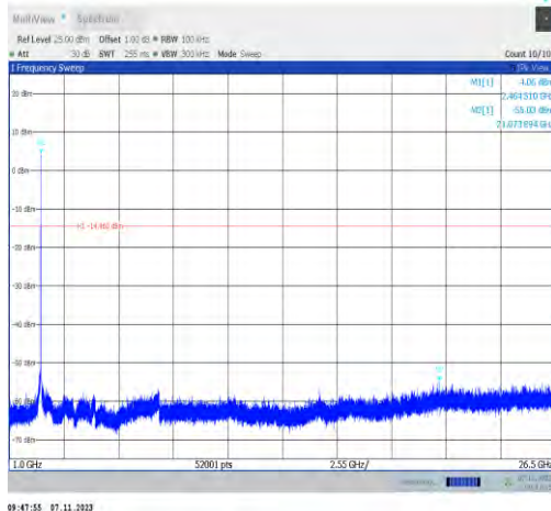
11n20SISO-Ant2-2462-1000~26500-PASS
