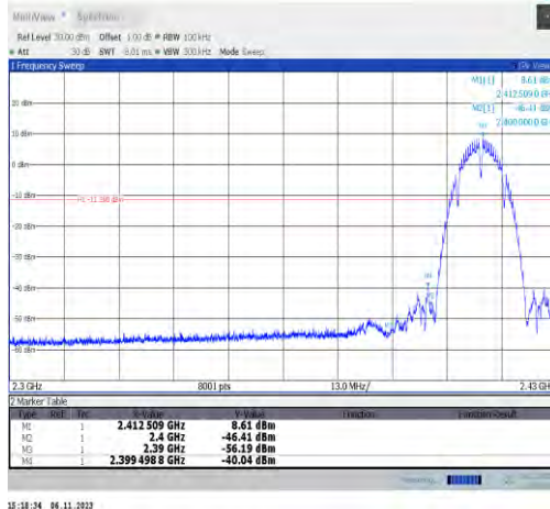
11b-Ant2-2412-PASS
