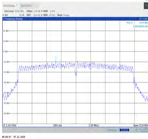
11n20ISO-Ant2-2412-PASS
