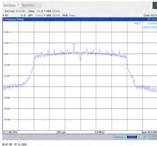
11n20SISO-Ant2-2462-0~Reference-PASS
