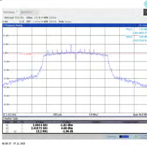
11n20SISO-Ant2-2412-PASS
