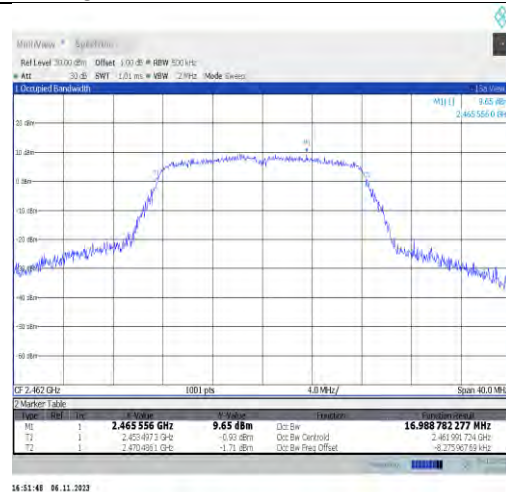
11g-Ant2-2462
