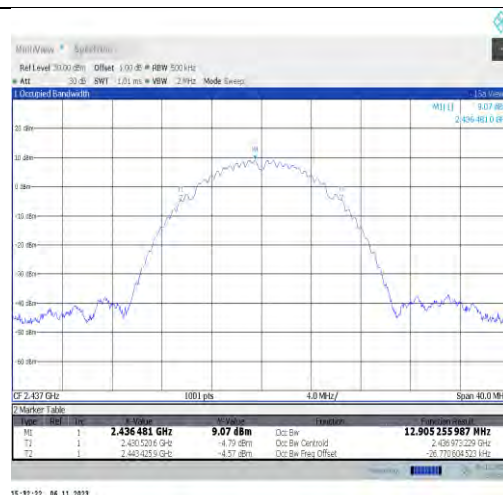
11b-Ant2-2437
