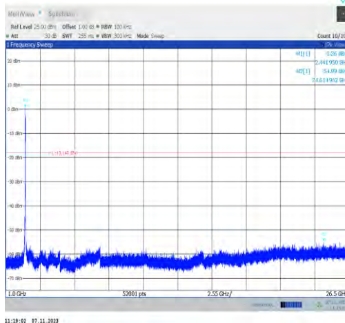
11n40SISO-Ant2-2437-1000~26500-PASS
