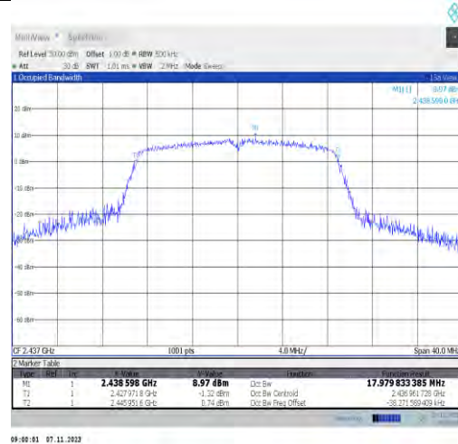
11n20SISO-Ant2-2437
