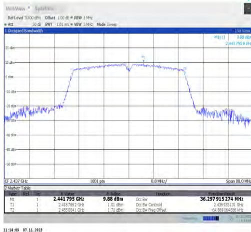
11n40SISO-Ant2-2437
