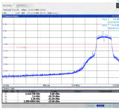
11g-Ant2-2412-PASS
