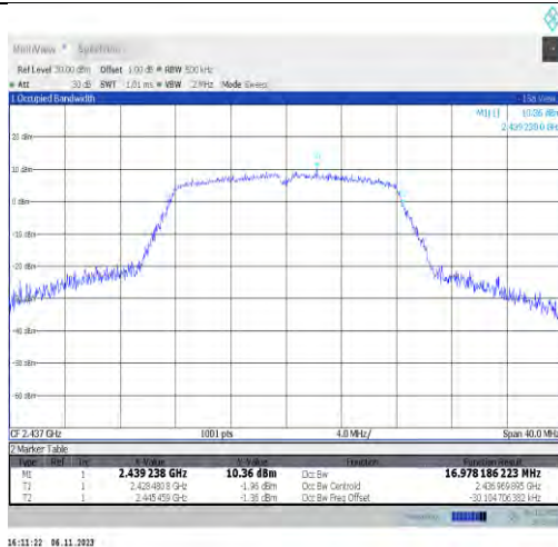
11g-Ant2-2437
