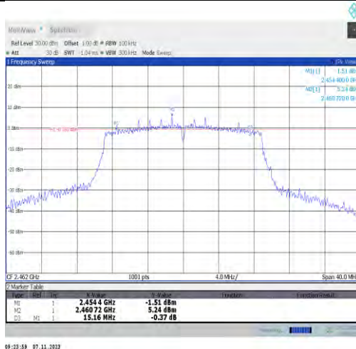
11n20SISO-Ant2-2462-PASS
