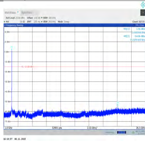
11g-Ant2-2412-1000~26500-PASS
