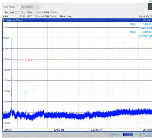
11b-Ant2-2462-1000~26500-PASS
