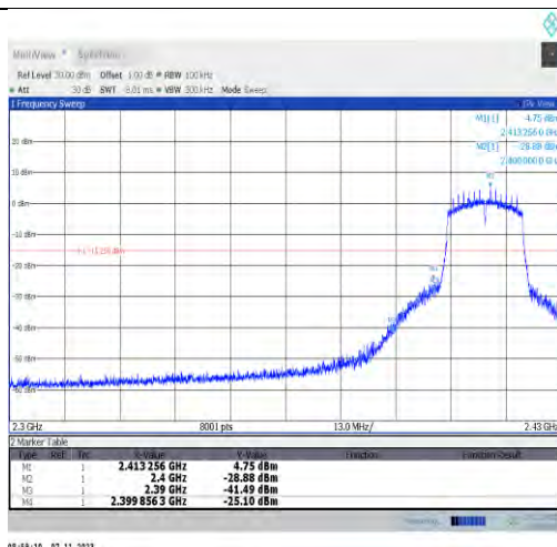
11n20ISO-Ant2-2412-PASS
