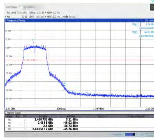
11g-Ant2-2462-PASS
