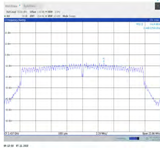
11n20ISO-Ant2-2437-PASS
