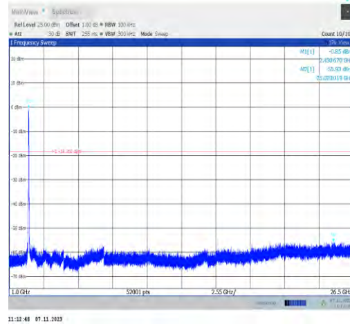
11n40SISO-Ant2-2422-1000~26500-PASS
