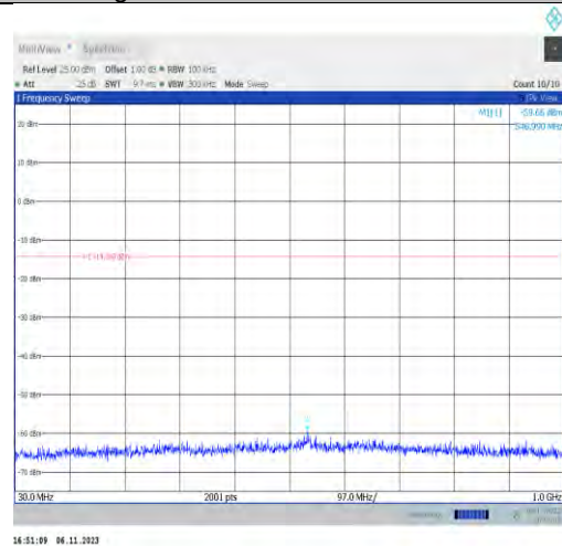
11g-Ant2-2437-30~1000-PASS
