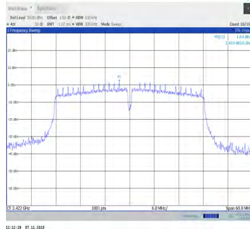
11n40SISO-Ant2-2422-0~Reference-PASS
