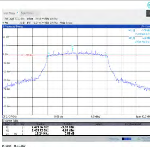
11g-Ant2-2437-PASS
