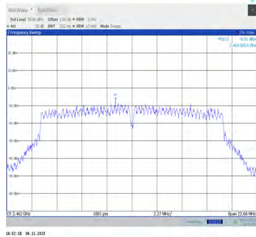
11g-Ant2-2462-PASS
