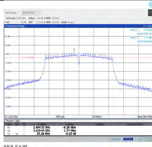
11n40SISO-Ant2-2422-PASS
