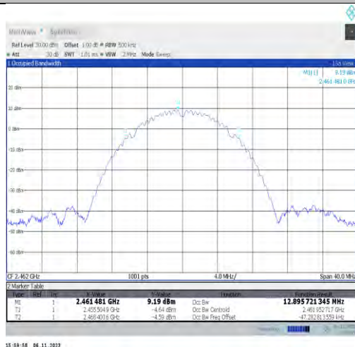
11b-Ant2-2462
