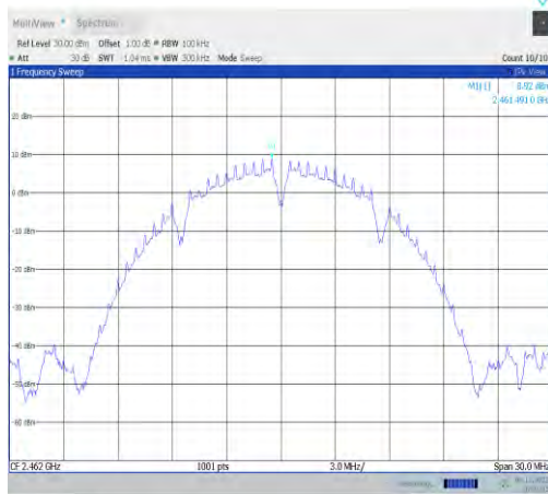
11b-Ant2-2462-0~Reference-PASS
