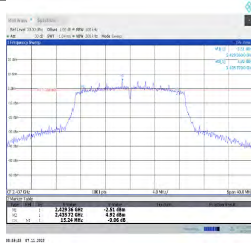
11n20SISO-Ant2-2437-PASS
