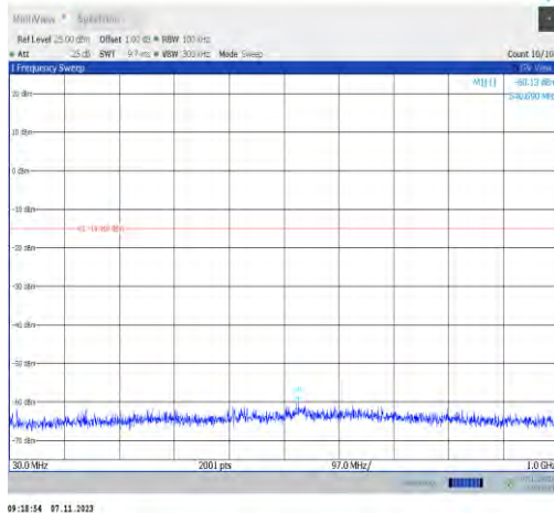
11n20SISO-Ant2-2437-30~1000-PASS
