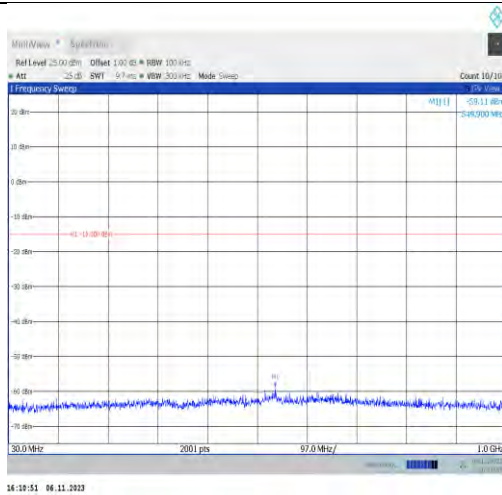
11g-Ant2-2412-30~1000-PASS
