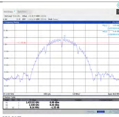
11b-Ant2-2437-PASS
