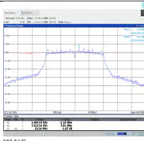
11g-Ant2-2412-PASS
