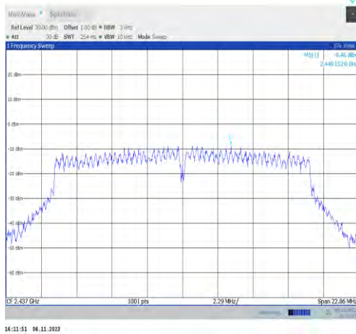
11g-Ant2-2437-PASS
