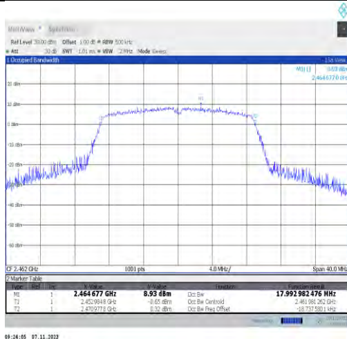
11n20SISO-Ant2-2462
