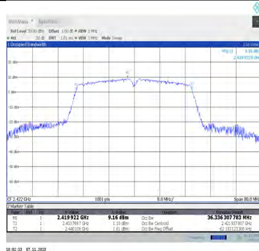
11n40SISO-Ant2-2422
