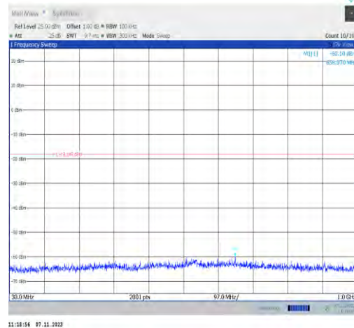
11n40SISO-Ant2-2437-30~1000-PASS
