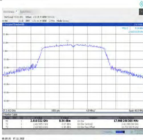
11n20SISO-Ant2-2412
