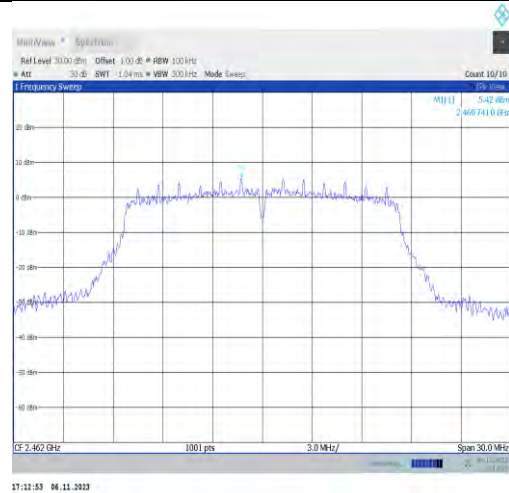
11g-Ant2-2462-0~Reference-PASS
