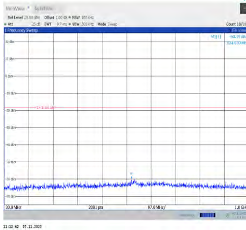
11n40SISO-Ant2-2422-30~1000-PASS
