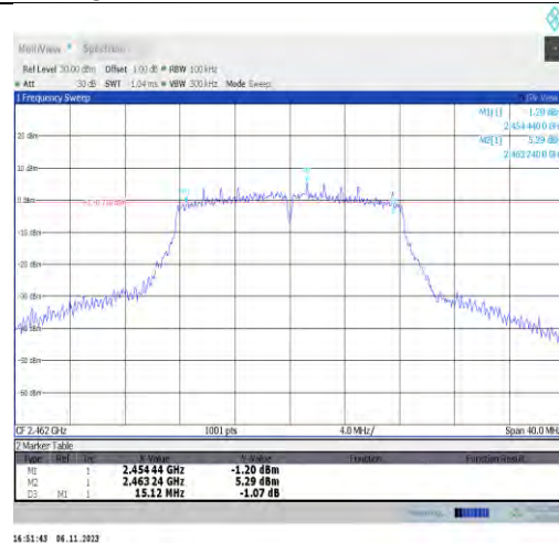
11g-Ant2-2462-PASS
