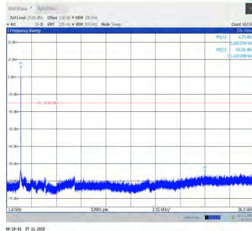
11n20SISO-Ant2-2437-1000~26500-PASS
