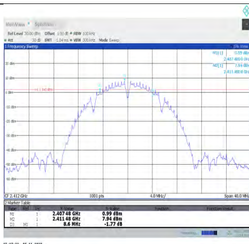
11b-Ant2-2412-PASS
