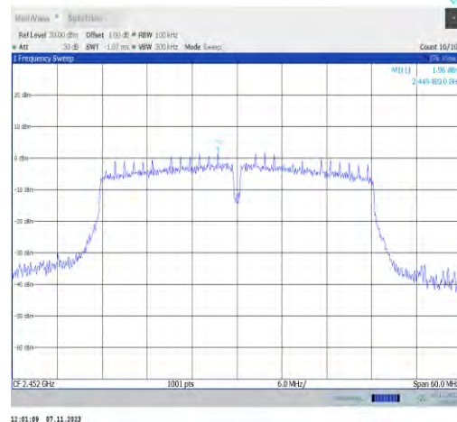
11n40SISO-Ant2-2452-0~Reference-PASS
