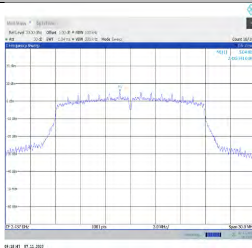
11n20SISO-Ant2-2437-0~Reference-PASS
