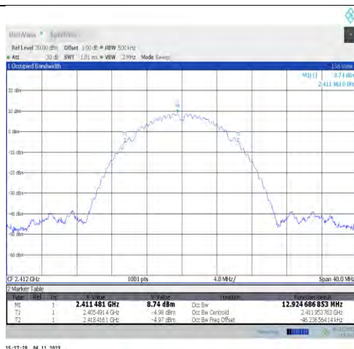
11b-Ant2-2412
