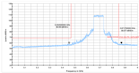
802.11ax HE80-Channel 138: Peak
