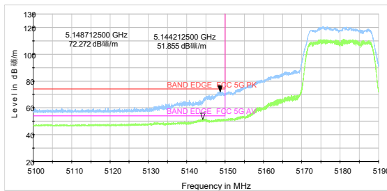
802.11n HT20-Channel 36: Peak + Average
