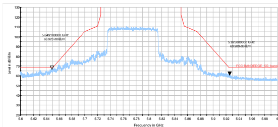
802.11ax HE80- Channel 155: Peak
