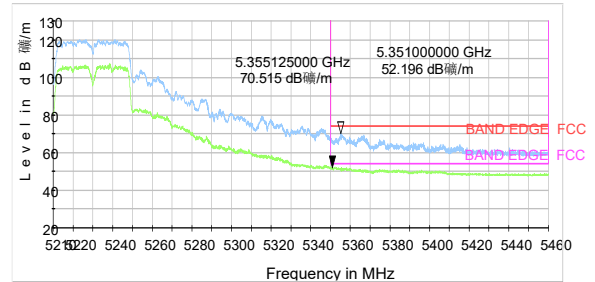
802.11n HT40-Channel 46: Peak + Average
