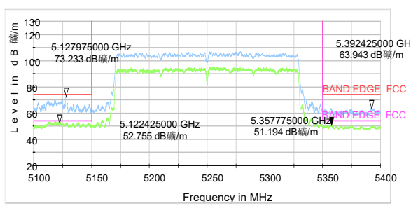
802.11ax HE160-Channel 50: Peak + Average
