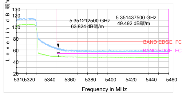
802.11ax HE40-Channel 62: Peak + Average
