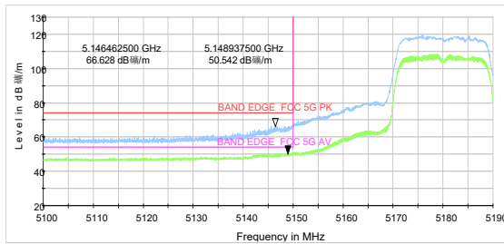
802.11n HT40-Channel 38: Peak + Average
