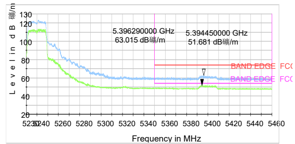
802.11n HT20-Channel 48: Peak + Average
