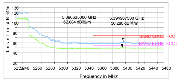
802.11n HT40-Channel 46: Peak + Average
