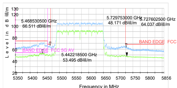
802.11ax HE160-Channel 114: Peak + Average
