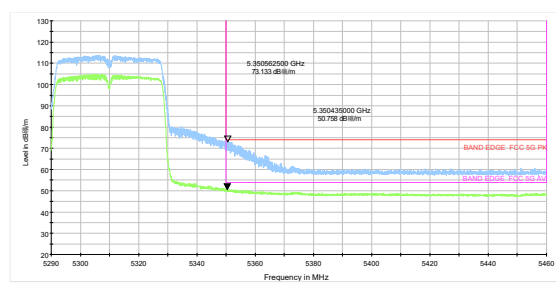
802.11ac VHT160 -Channel 50: Peak + Average
