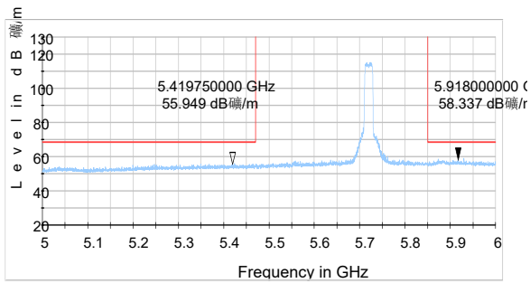
802.11n HT20-Channel 140: Peak
