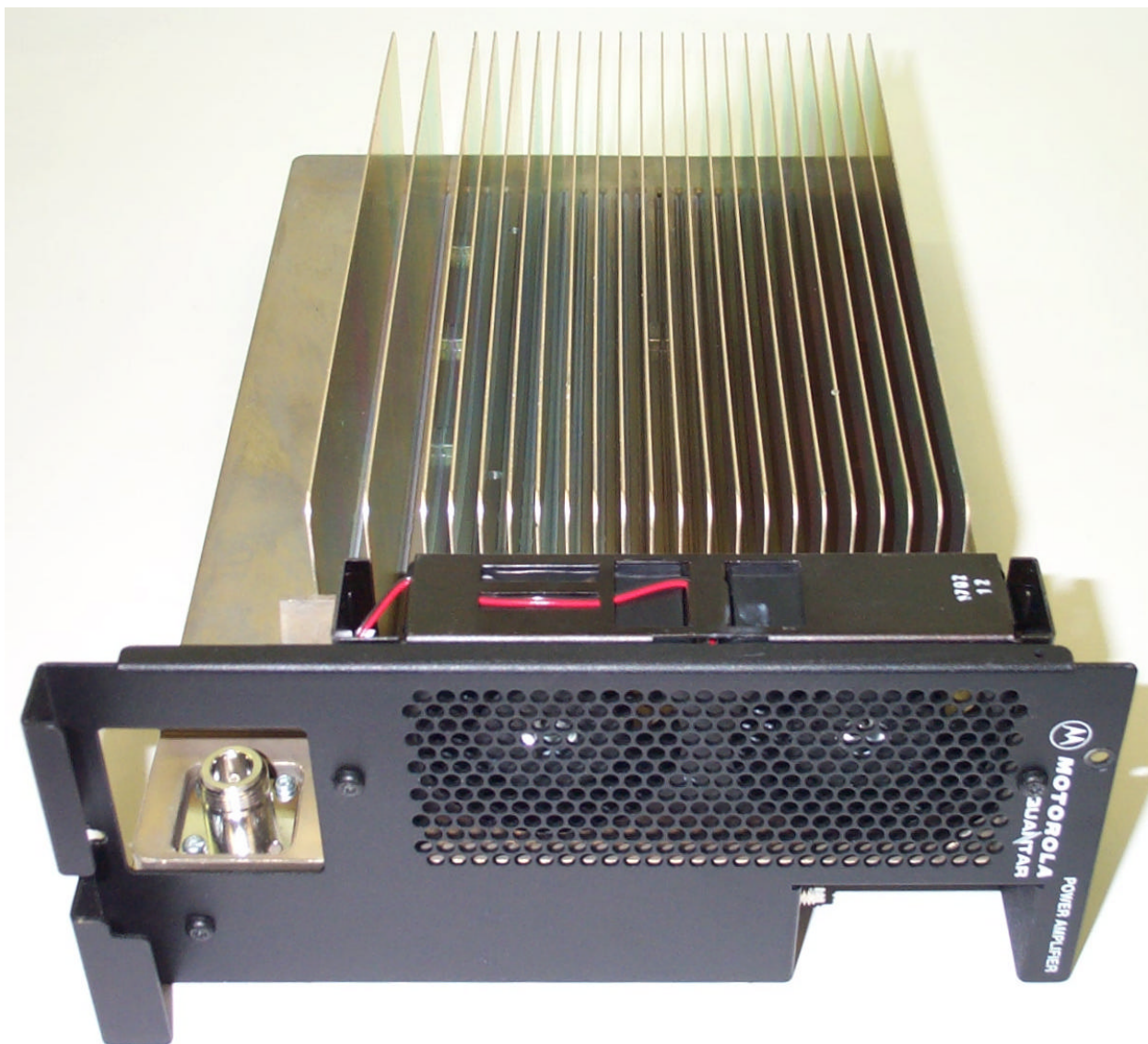
Power Amplifier Module, Heat Sink View
