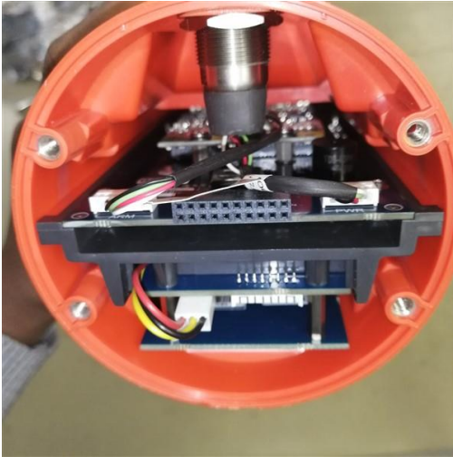
Photo 1: Internal view
