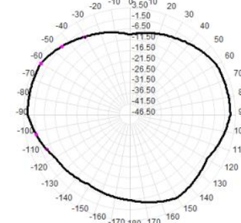
2450.0MHz Total(H-XY), Max= 1.66dBi
