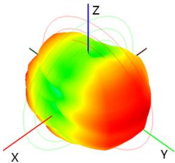
2450.0MHz H+V, Eff: 50.9%
