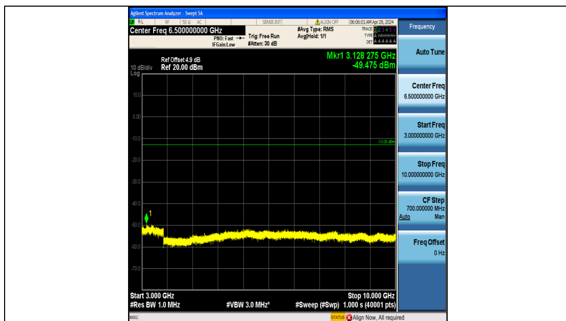
Band5_10MHz_QPSK_20525_50RB#0_3000~10000_3000~10000
