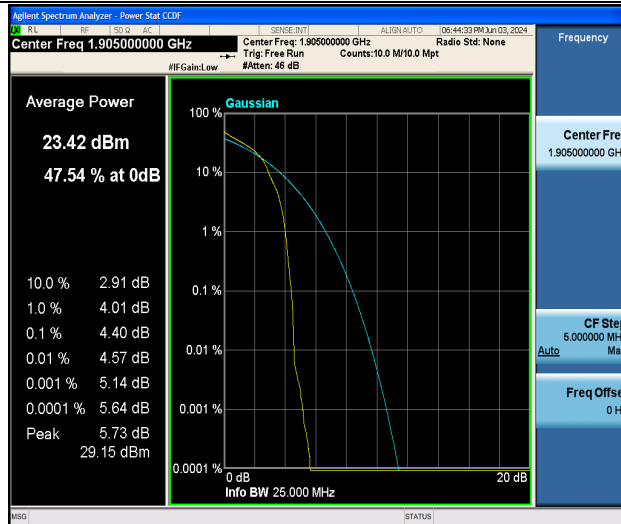
Band25-20MHz-16QAM-26590-1RB#0-PASS
