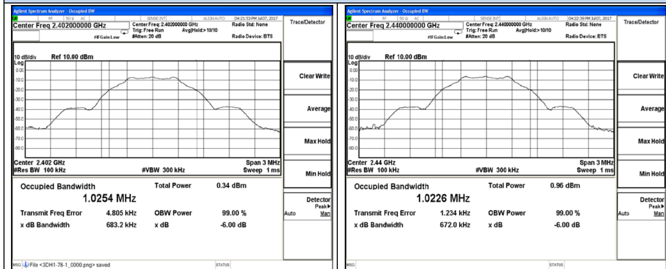
Channel 0 / 2402 MHz
