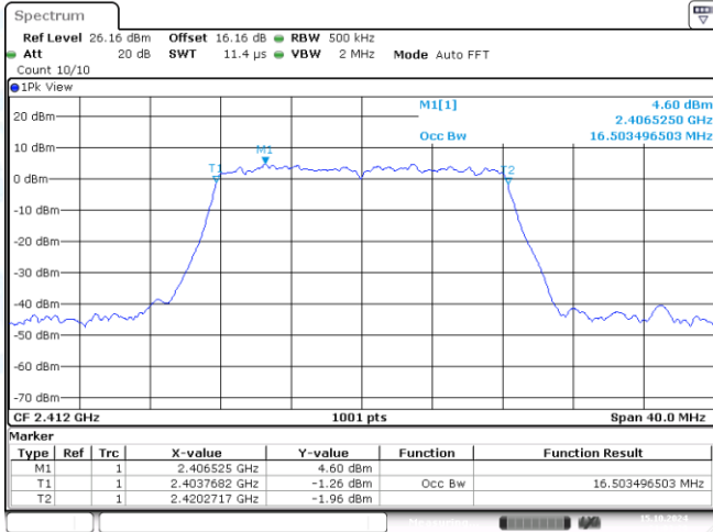
11G-CDD-Ant1-2412
