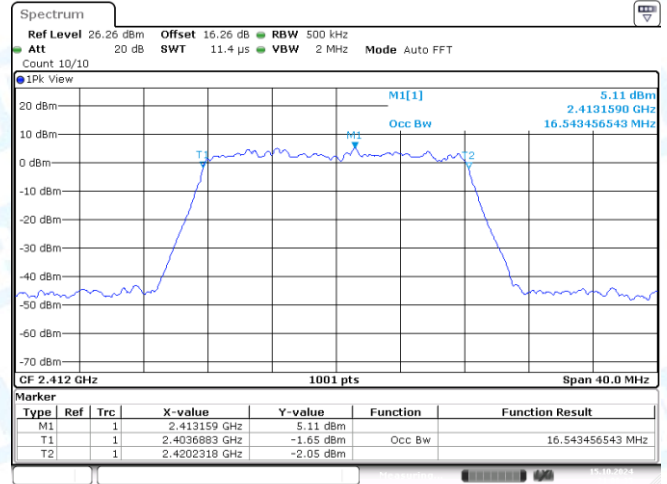
11G-CDD-Ant2-2412
