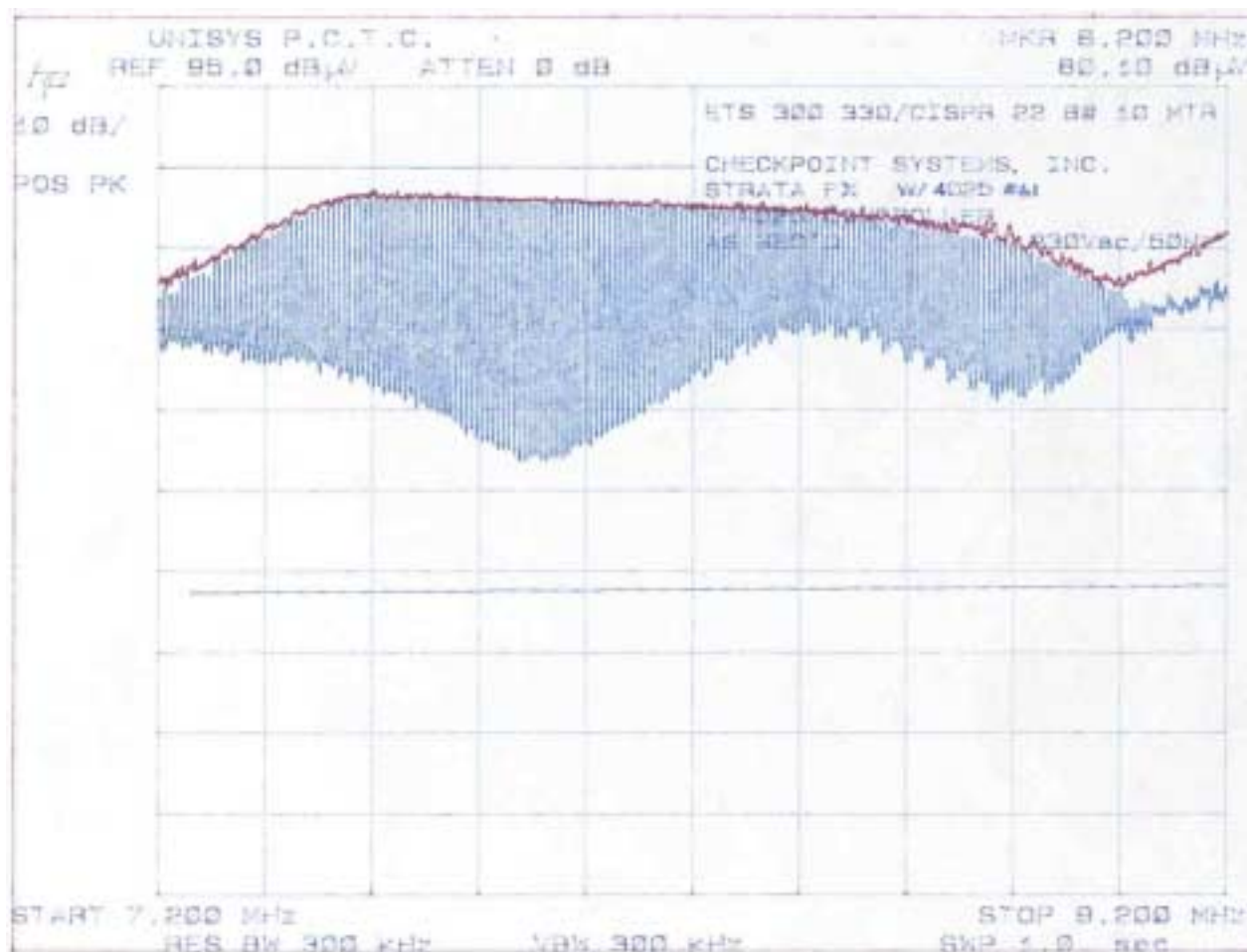
Photo 5 – Bandwidth Plot
