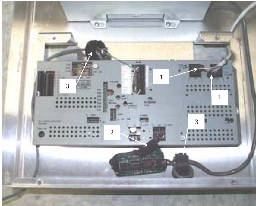
Photo 2 – Ferrite Locations
