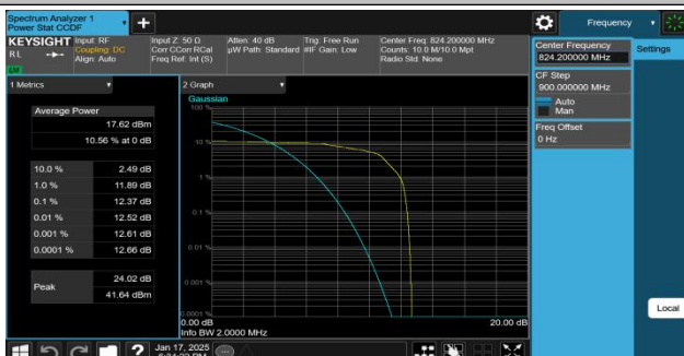
EGPRS850-128-8-PASS
