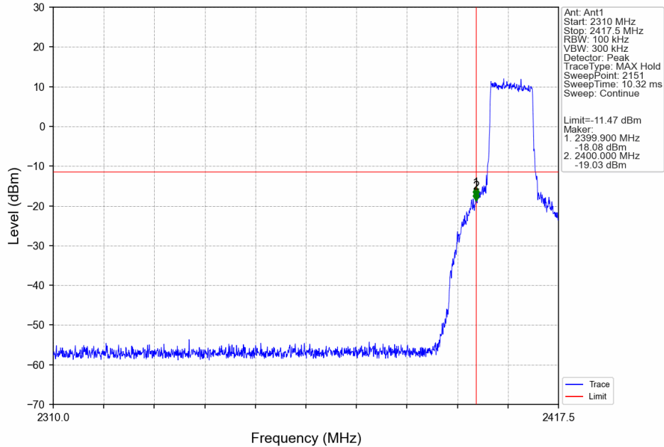
10M_LCH_2407.5MHz_Ant1_NTNV
