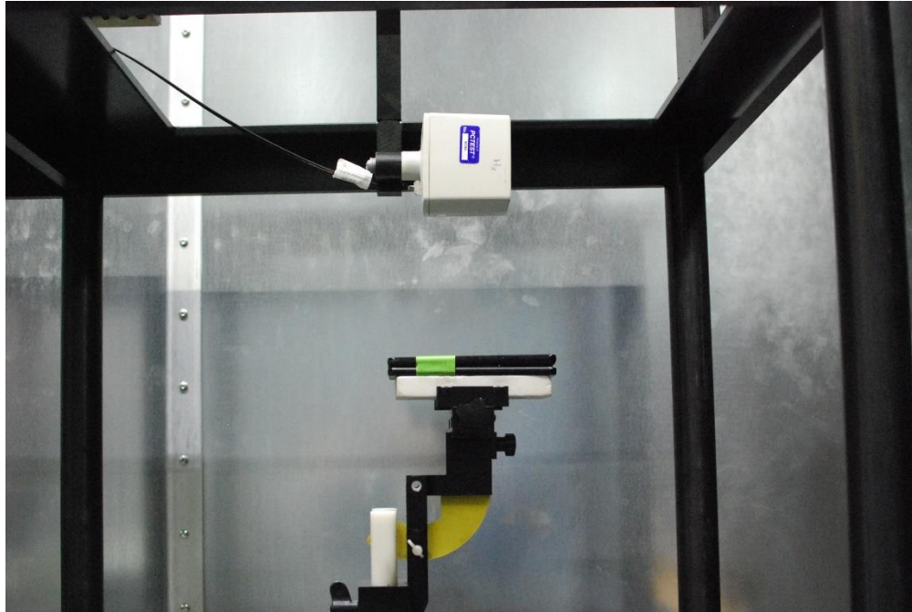
Photo 5. E-field 15cm
