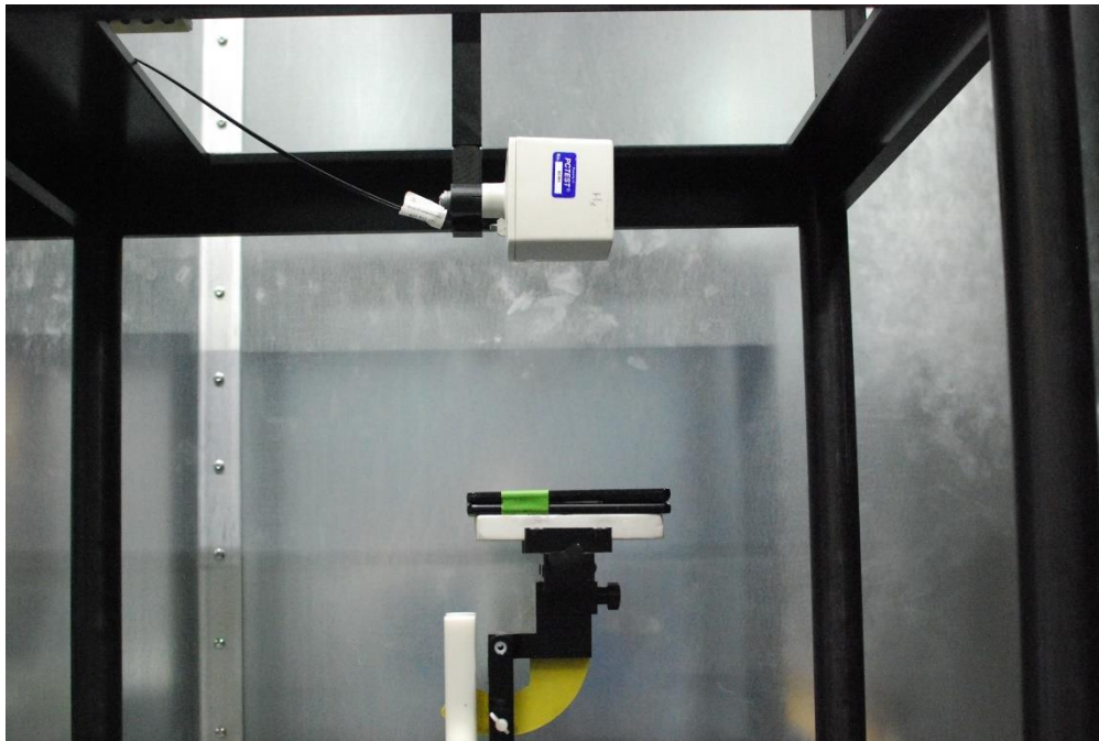
Photo 10. E-field 20cm
