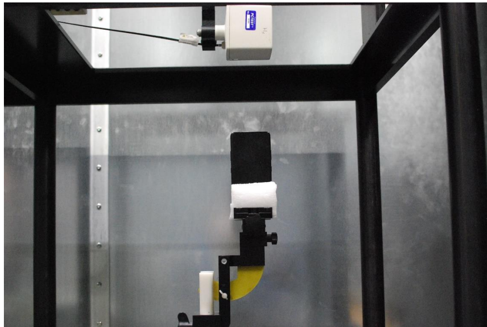
Photo 6. E-field 15cm
