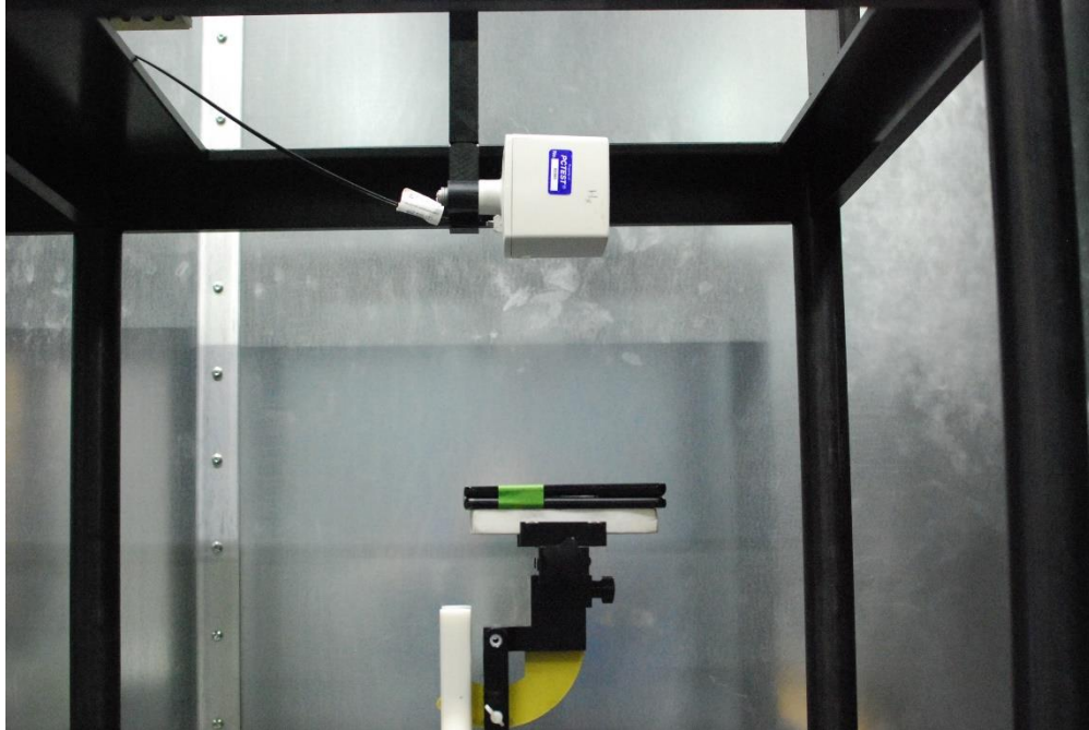
Photo 9. E-field 20cm
