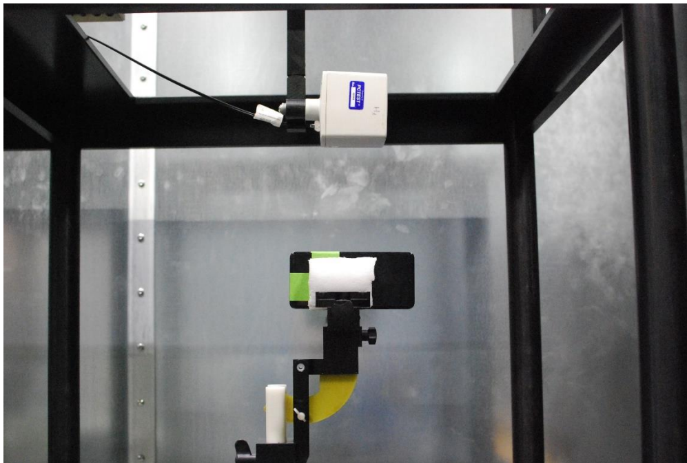
Photo 2. E-field 15cm
