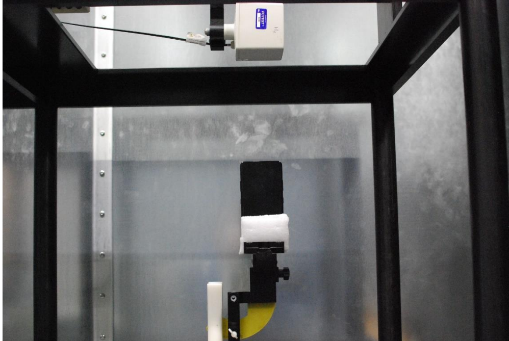
Photo 11. E-field 20cm
