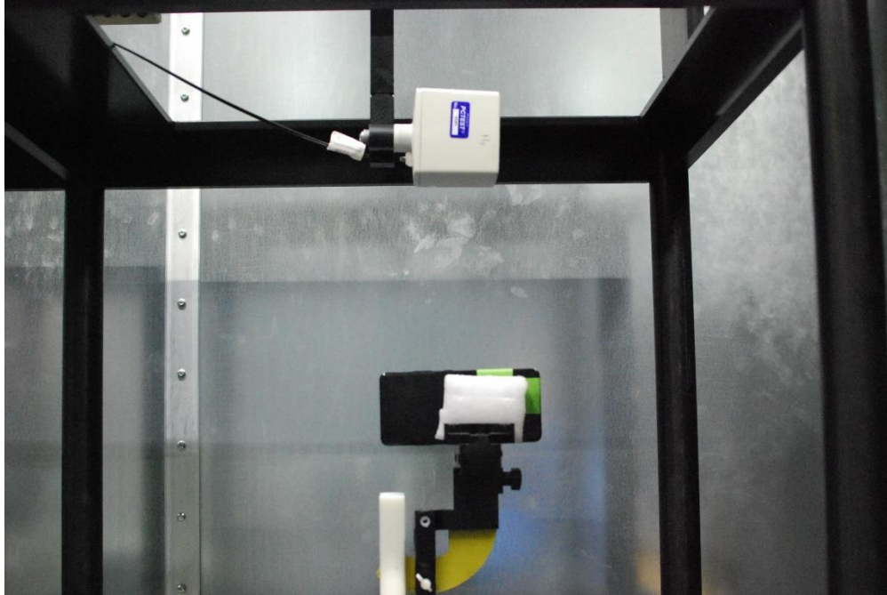
Photo 7. E-field 20cm
