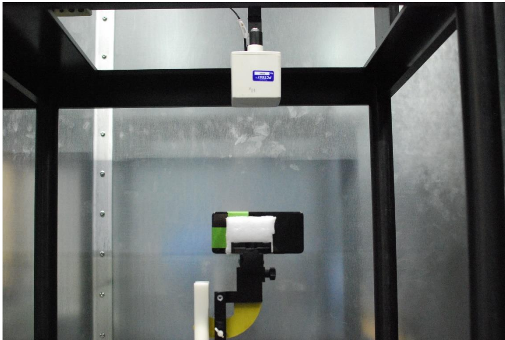
Photo 20. H-field 20cm
