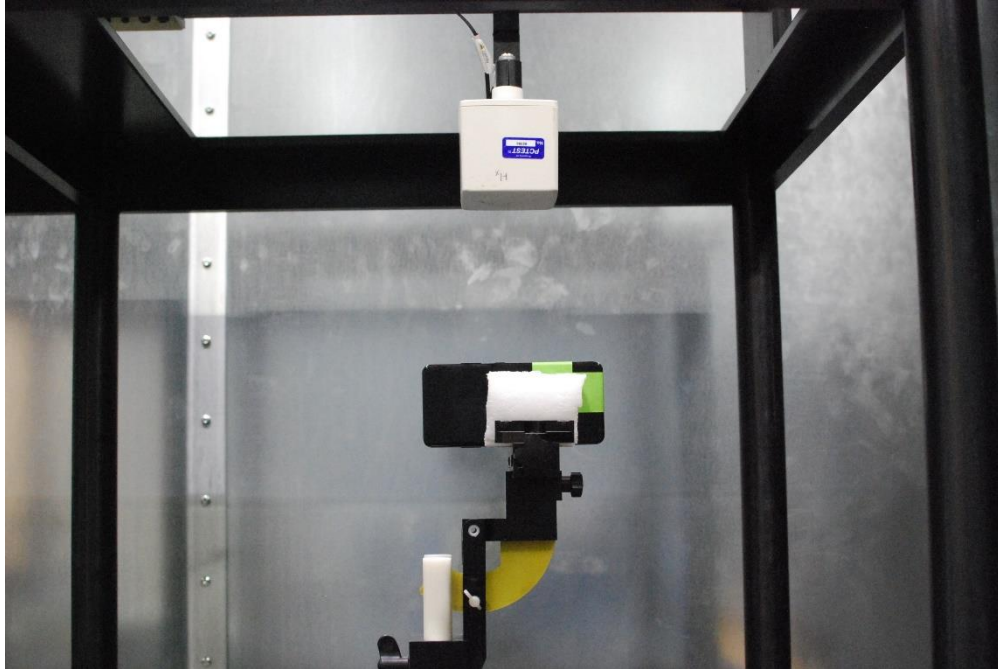
Photo 13. H-field 15cm
