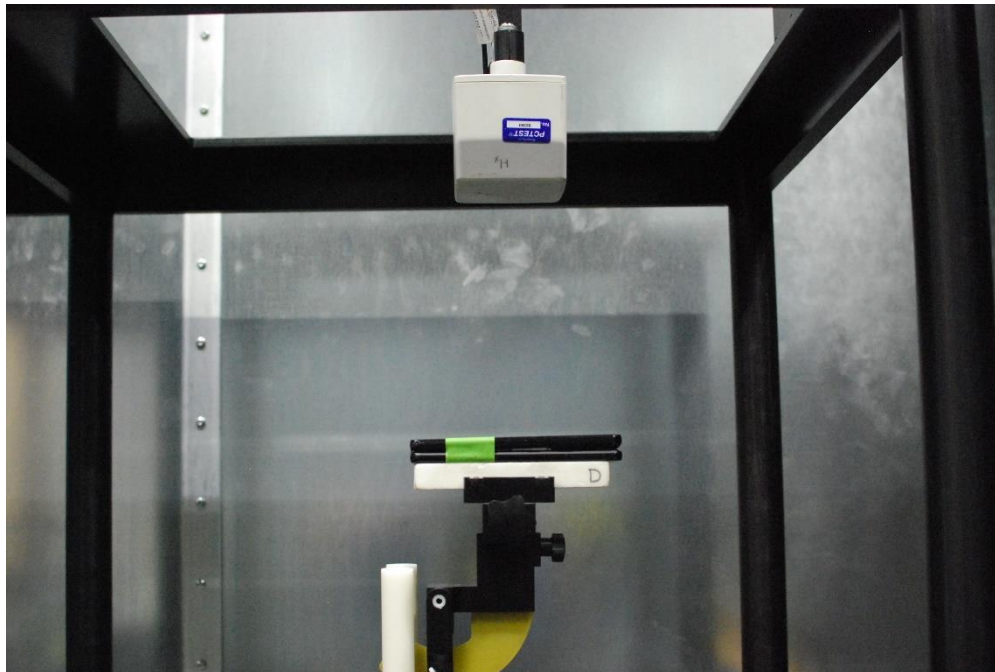
Photo 21. H-field 20cm
