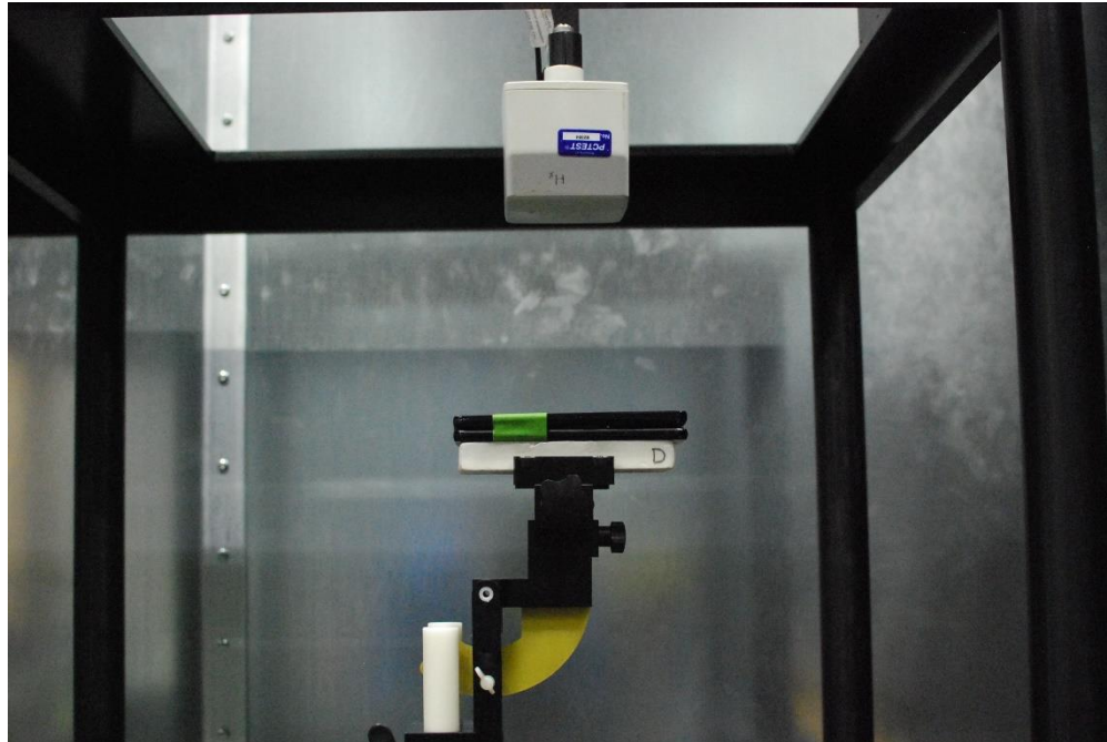
Photo 17. H-field 15cm
