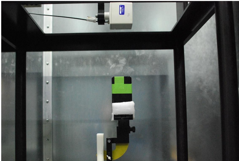
Photo 12. E-field 20cm
