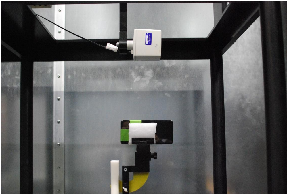
Photo 8. E-field 20cm
