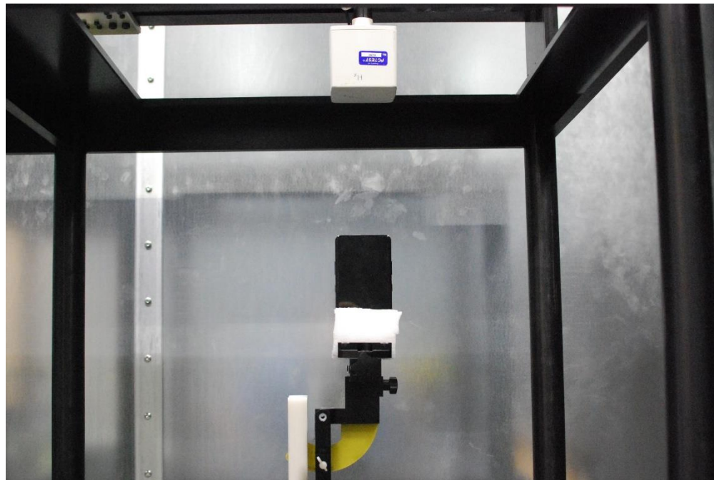
Photo 24. H-field 20cm
