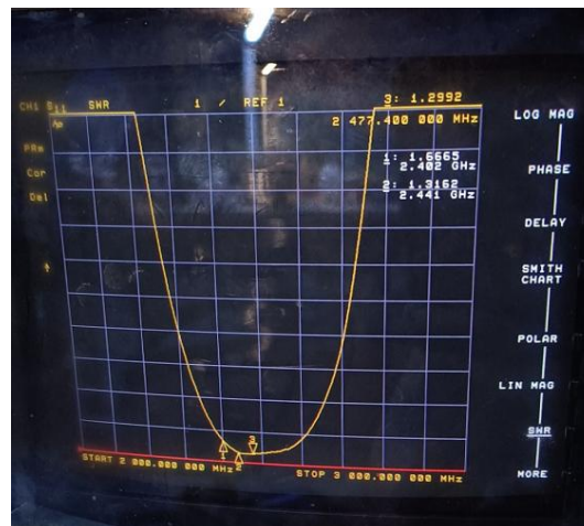
(c) VSWR
