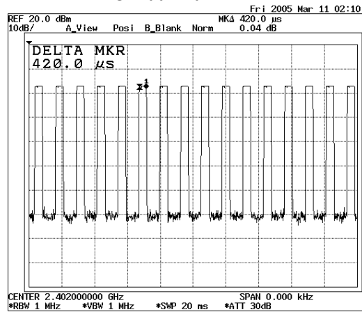
CH 00 2402MHz
