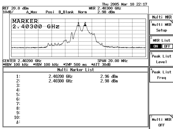
Channel 00 2402MHz
