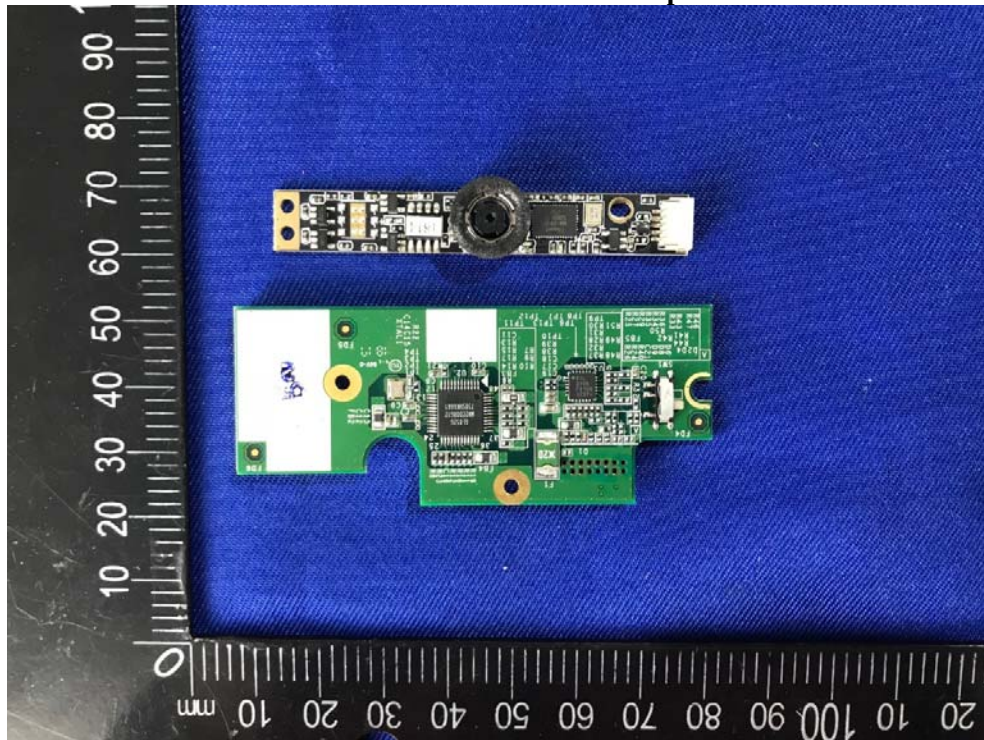
EUT – 2.4G Module Sun-board Top View
