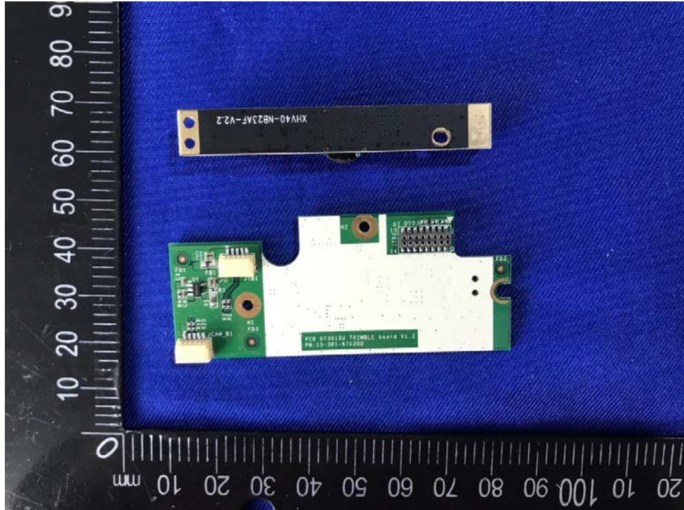
EUT – 2.4G Module Sun-board Bottom View
