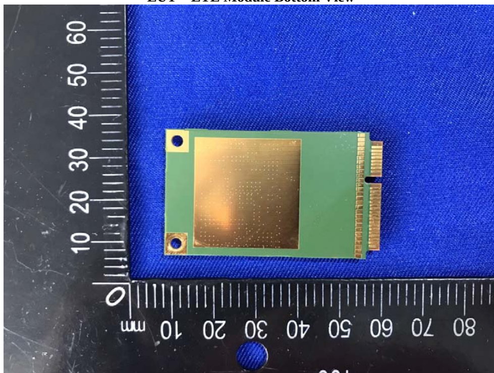
EUT – LTE Module Bottom View
