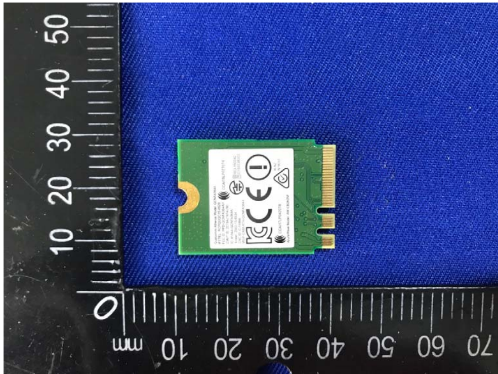
EUT – WIFI Module Bottom View
