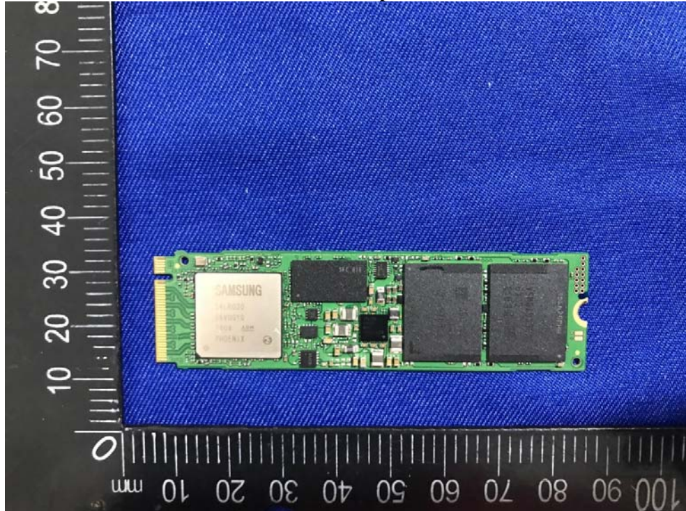
EUT – SSD Top View
