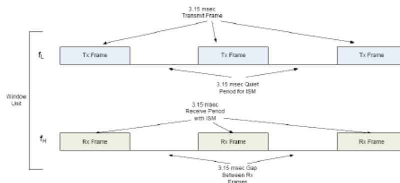
Figure 3 - Channel Loading During CU Synchronization Mode
