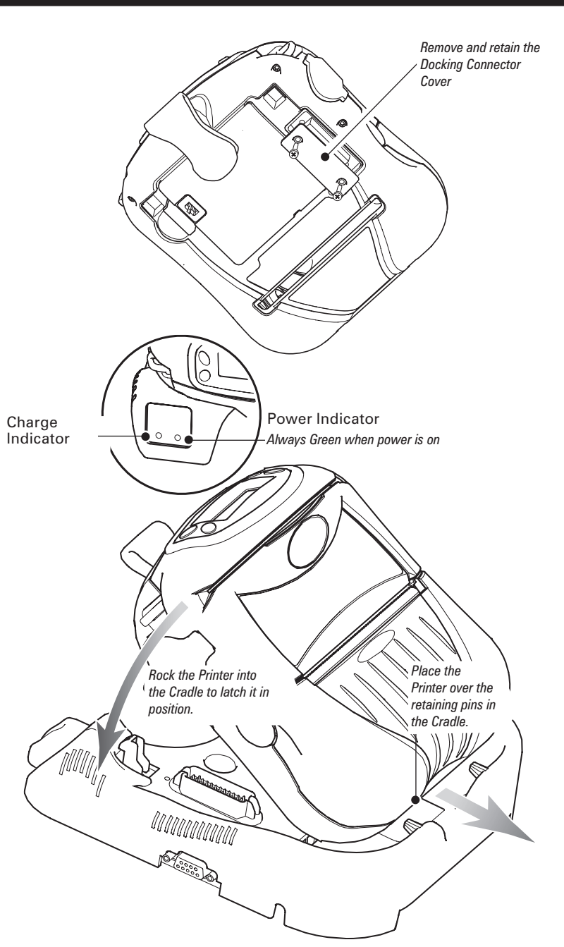
Figure 20: Installing the Printer into the Cradle
