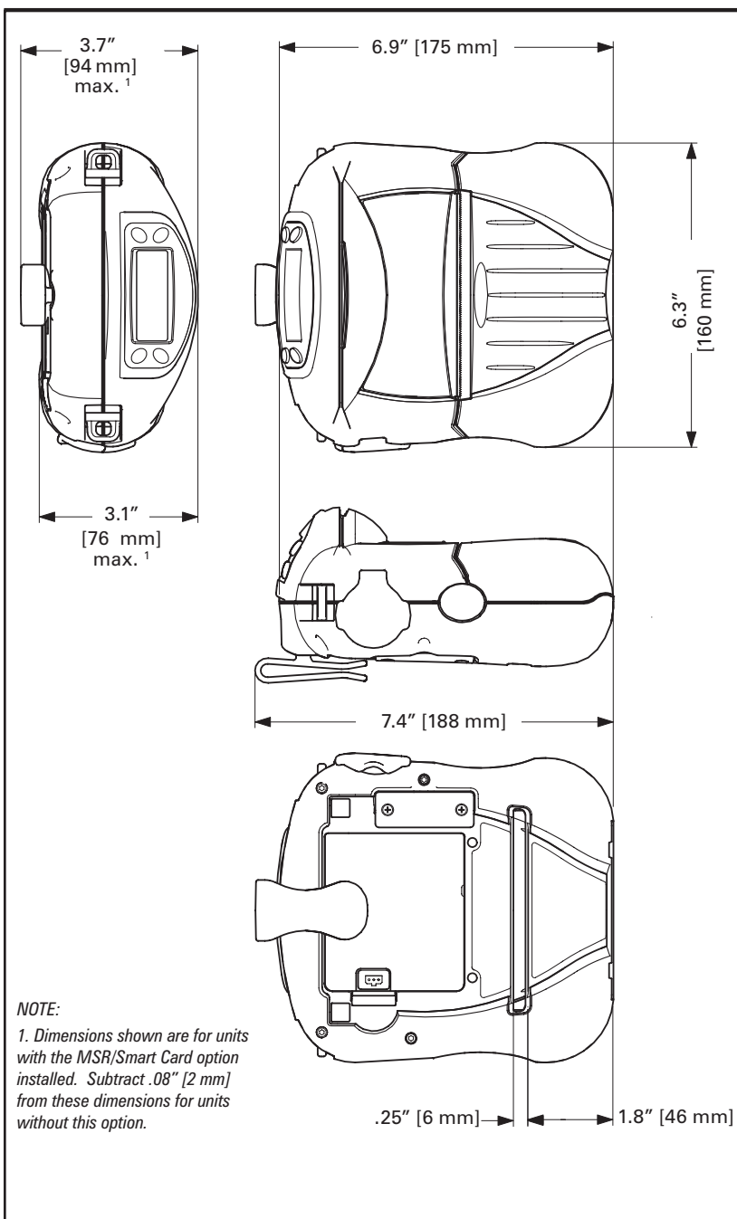
Figure 25: RW 420 Overall Dimensions
