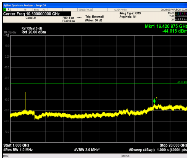
Band38_10MHz_QPSK_38000_1RB#0_1000~20000_1000~20000
