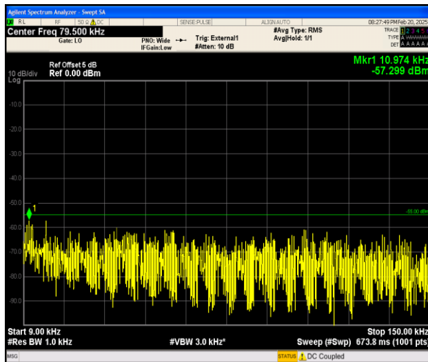
Band38_10MHz_16QAM_38200_1RB#0_0.009~0.15_0.009~0.15
