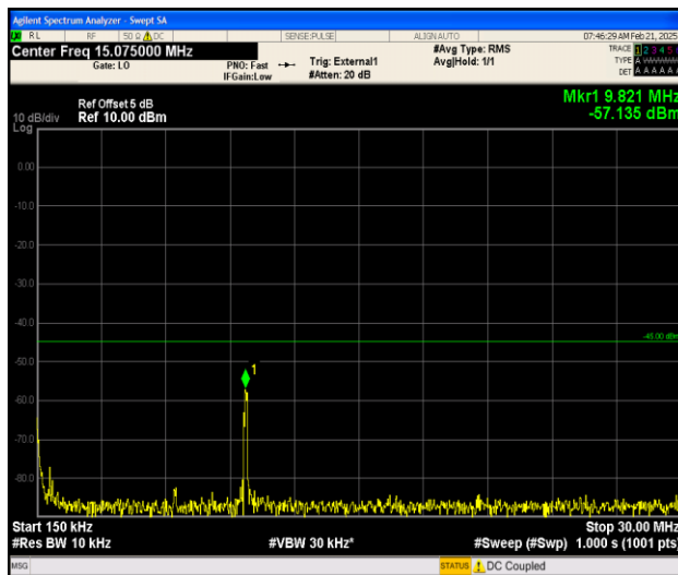
Band38_20MHz_QPSK_37850_1RB#0_0.15~30_0.15~30
