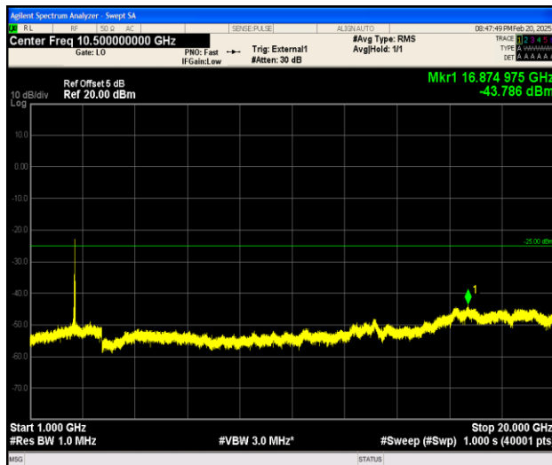
Band38_15MHz_16QAM_38175_1RB#0_1000~20000_1000~20000
