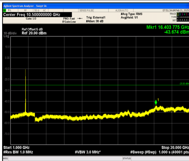
Band38_20MHz_QPSK_38150_1RB#0_1000~20000_1000~20000
