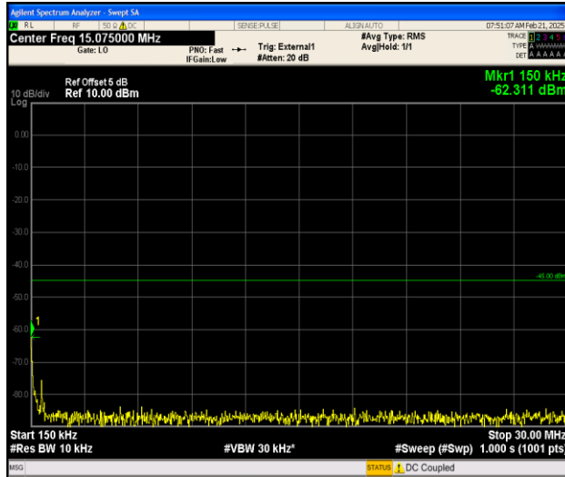
Band38_20MHz_QPSK_38150_1RB#0_0.15~30_0.15~30
