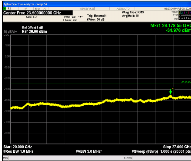
Band38_10MHz_QPSK_38200_1RB#0_20000~27000_20000~27000
