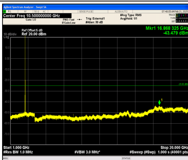
Band38_20MHz_16QAM_37850_1RB#0_1000~20000_1000~20000
