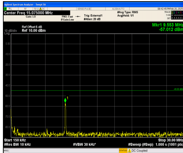
Band38_15MHz_16QAM_37825_1RB#0_0.15~30_0.15~30
