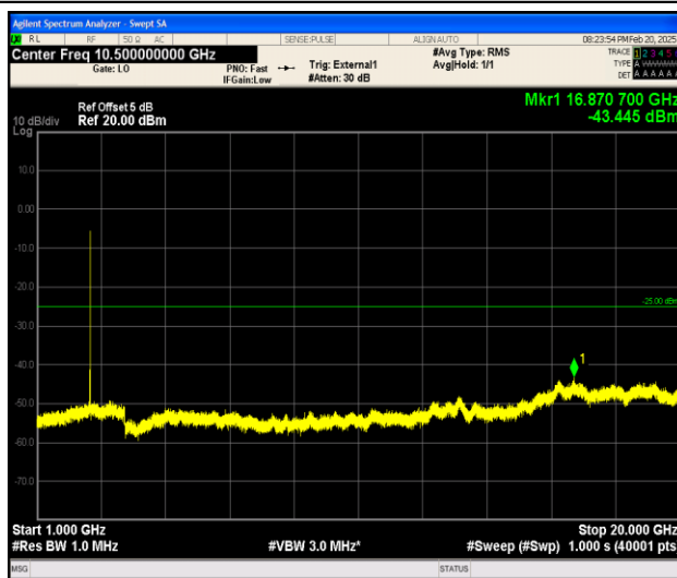
Band38_10MHz_16QAM_37800_1RB#0_1000~20000_1000~20000
