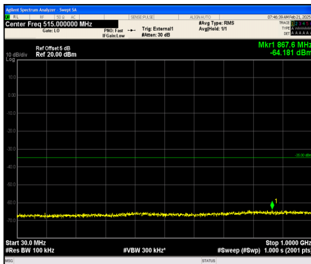
Band38_20MHz_QPSK_37850_1RB#0_30~1000_30~1000
