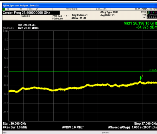
Band38_10MHz_QPSK_38000_1RB#0_20000~27000_20000~27000
