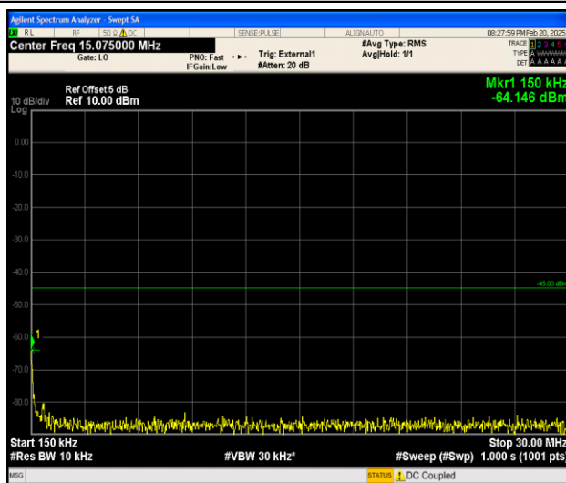
Band38_10MHz_16QAM_38200_1RB#0_0.15~30_0.15~30
