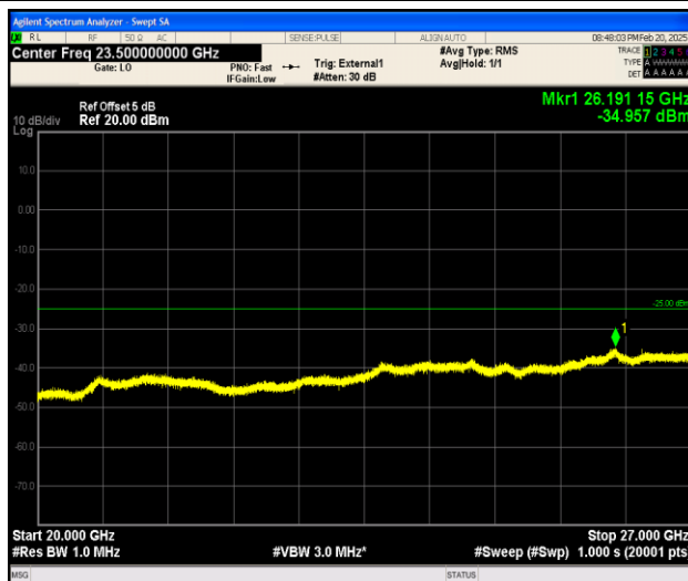
Band38_15MHz_16QAM_38175_1RB#0_20000~27000_20000~27000
