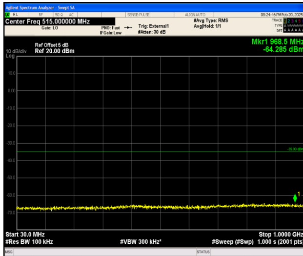
Band38_10MHz_QPSK_38000_1RB#0_30~1000_30~1000
