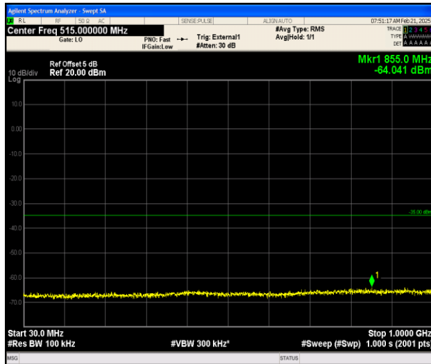
Band38_20MHz_QPSK_38150_1RB#0_30~1000_30~1000
