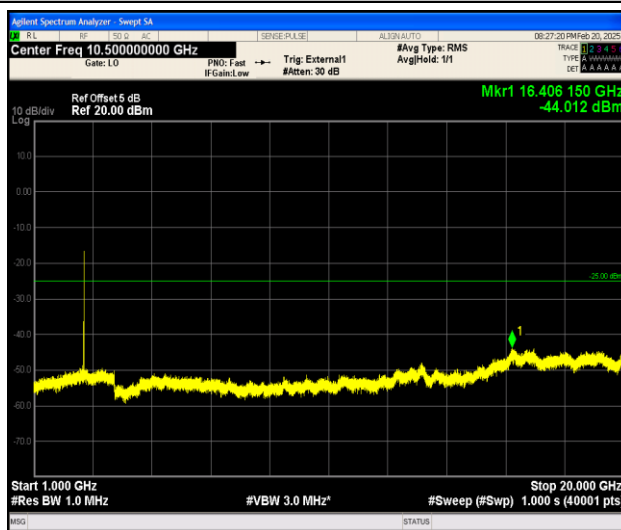
Band38_10MHz_QPSK_38200_1RB#0_1000~20000_1000~20000
