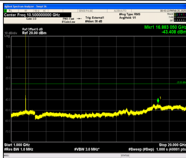
Band38_15MHz_16QAM_37825_1RB#0_1000~20000_1000~20000
