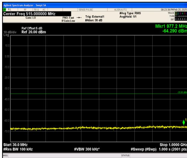
Band38_10MHz_16QAM_37800_1RB#0_30~1000_30~1000
