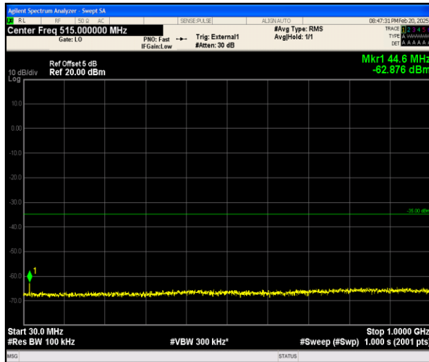
Band38_15MHz_16QAM_38175_1RB#0_30~1000_30~1000
