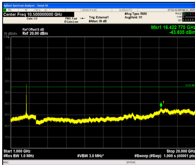
Band38_20MHz_16QAM_38150_1RB#0_1000~20000_1000~20000
