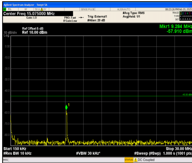
Band38_10MHz_16QAM_37800_1RB#0_0.15~30_0.15~30
