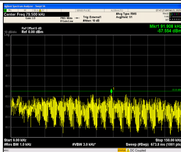
Band38_20MHz_16QAM_37850_1RB#0_0.009~0.15_0.009~0.15
