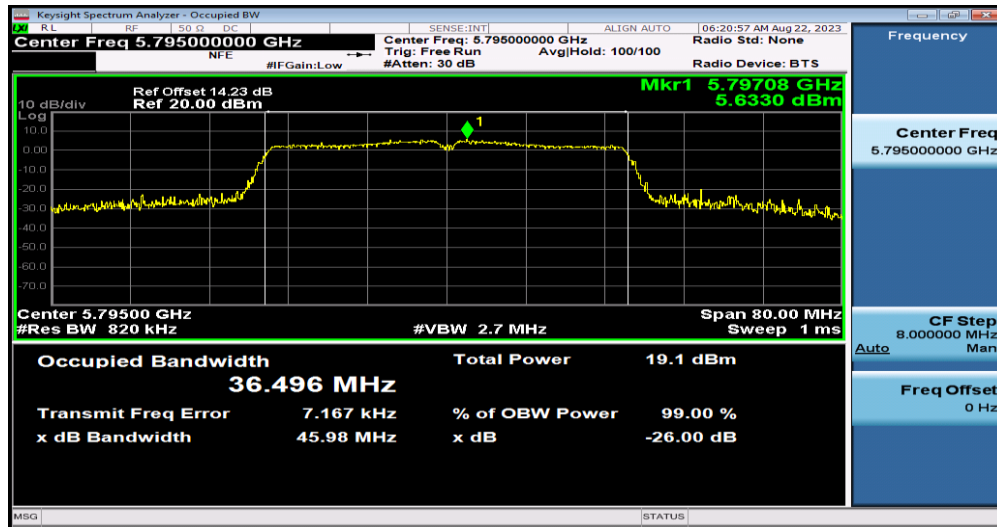
11AC40SISO-Ant1-5795
