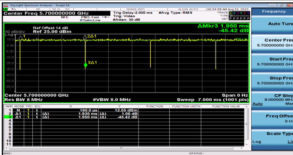
NTNV-11AC20SISO-Ant1-5700
