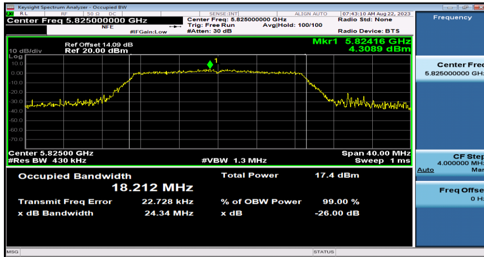
11AC20SISO-Ant1-5825
