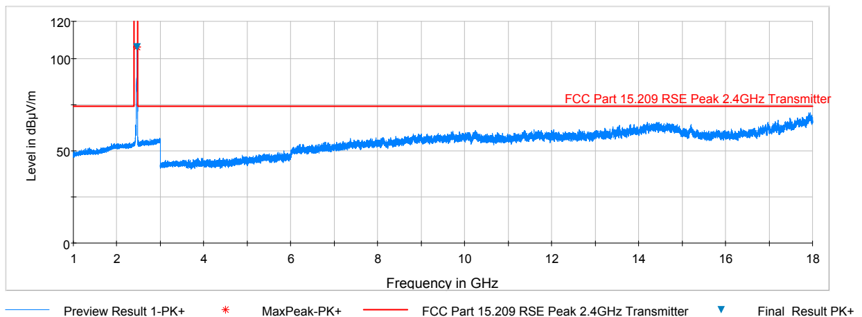
Plot 7-6. Radiated Spurious Plot above 1GHz (BT – Ch. 78, Ant. Pol. V)
