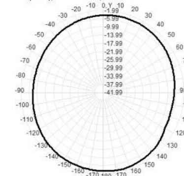
Total(H-XY), Max=-3.36dBi, CirD=4.65
