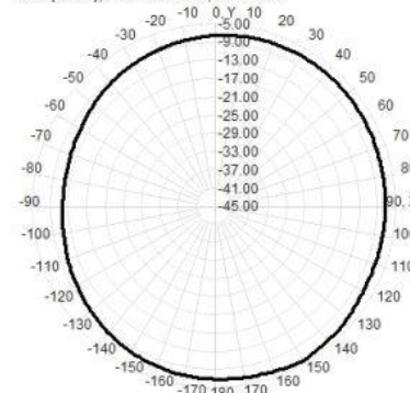
Total(H-XY), Max=-6.05dBi, CirD=5.72
