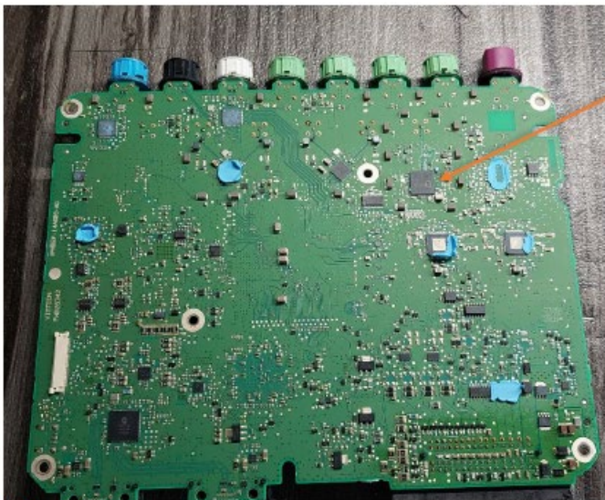
PCBA (bottom)
