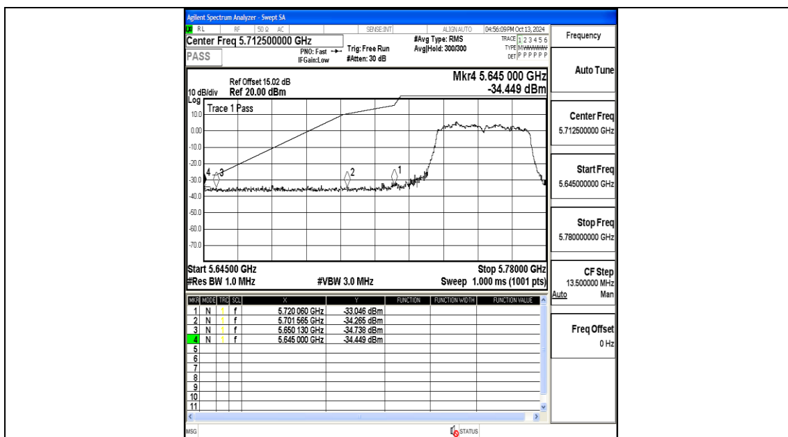
11AC40MIMO-Ant2-5755-PASS
