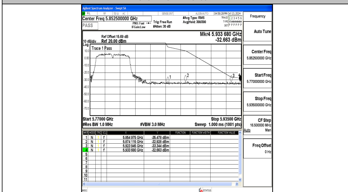
11AC40MIMO-Ant1-5795-PASS
