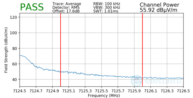
Plot 7-648. Antenna WF5t Radiated Upper Band Edge (Average – UNII Band 8)
