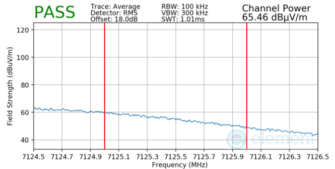
Plot 7-678. Antenna WF5b Radiated Upper Band Edge (Average – UNII Band 8)
